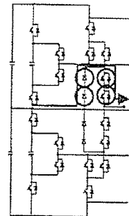
0 OUTPUT
