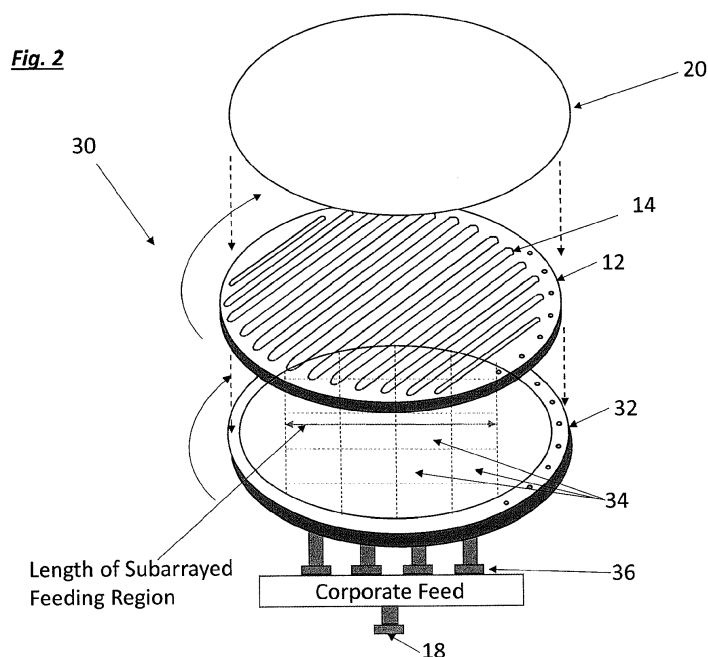
VICTS Antenna with subarrayed feeding
