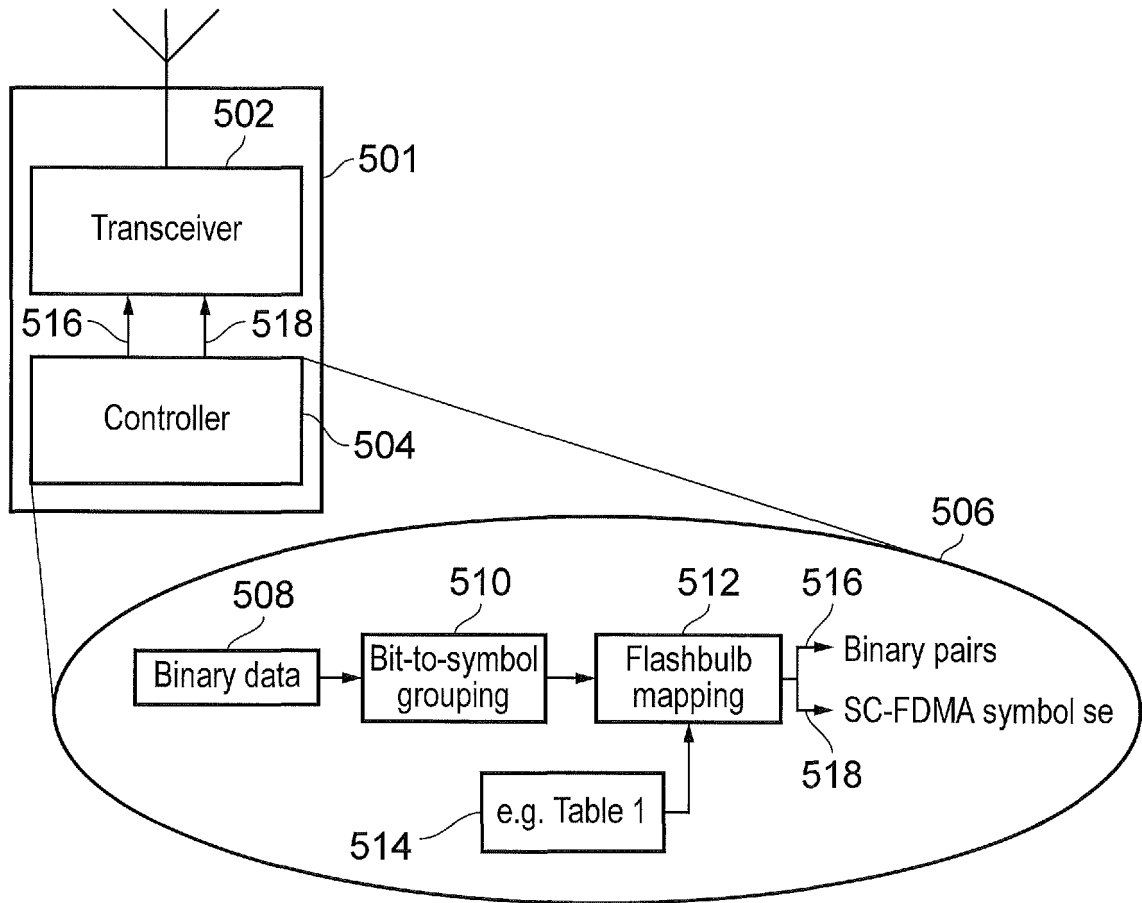
UE steps of flashlight transmission.
