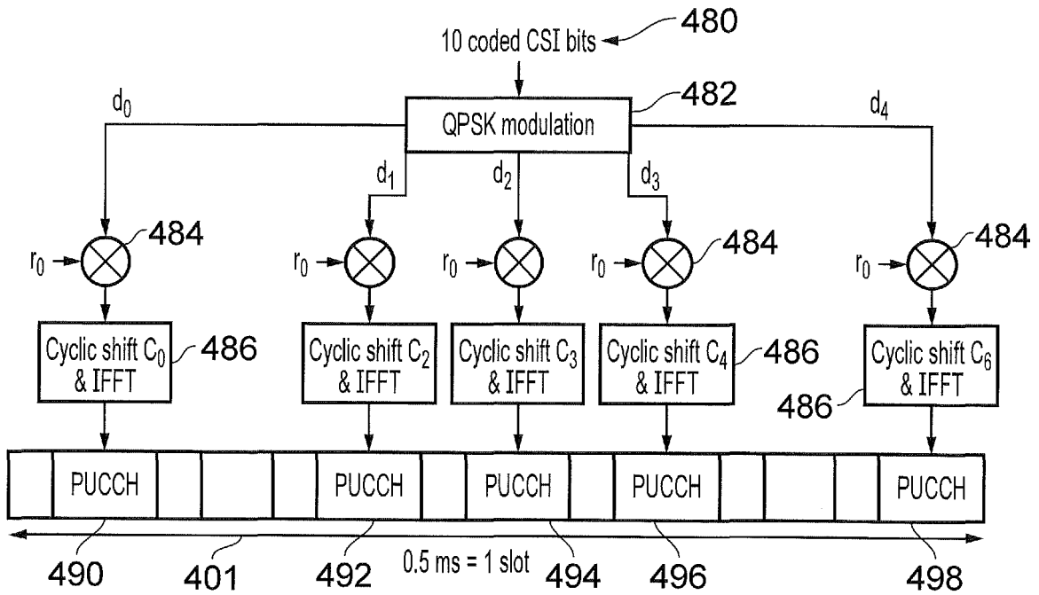
PUCCH format 2/2a/2b transmission and DM-RS, for normal cyclic-prefix operation. r_0 is a length-12 spreading code. The second slot takes d_5 through d_9 .
