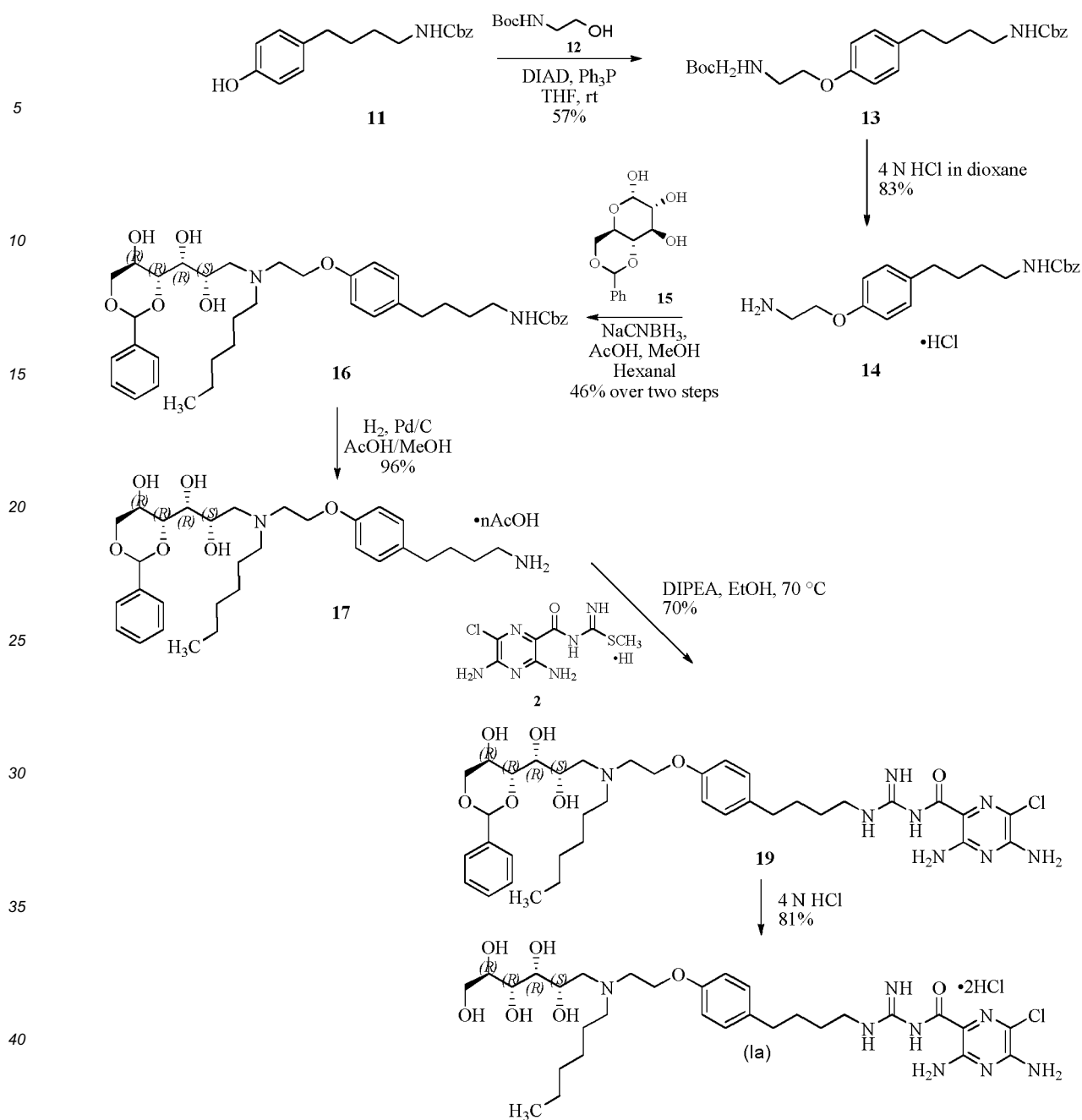
Scheme 3. Alternate Preparation of 3,5-Diamino-6-chloro-N-(N-(4-(4-(2-(hexyl((2S,3R,4R,5R)-2,3,4,5,6-pentahydroxyhexyl)amino)ethoxy)phenyl) butyl)carbamimidoyl)pyrazine-2-carboxamide
