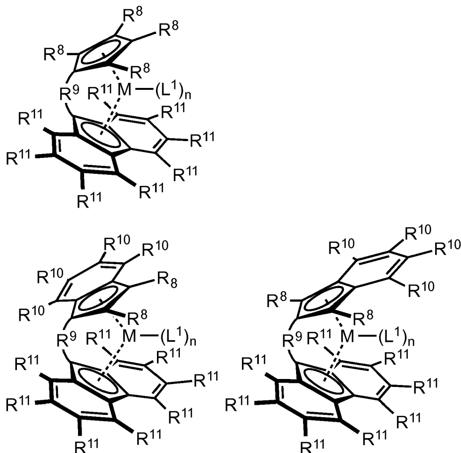
Formula XI
