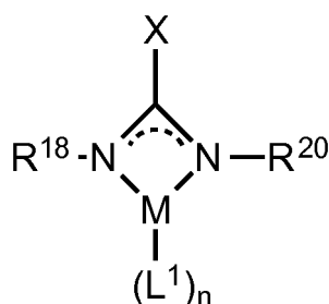
[R^{18}NC(X)NR^{20}]ML^1_n (Formula XX):
