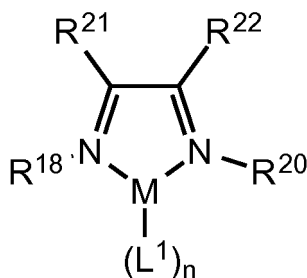
[R^{18}N=C(R^{21})C(R^{22})=NR^{20}]ML_n^1 (Formula XXI)
