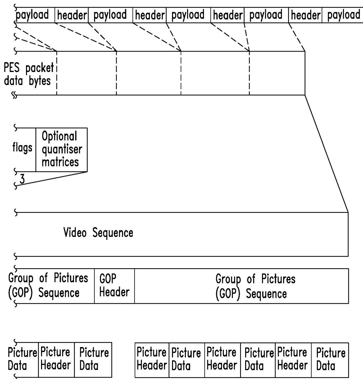
Figure 12(Continued) Parsing for bit_rate_value and stream_id
