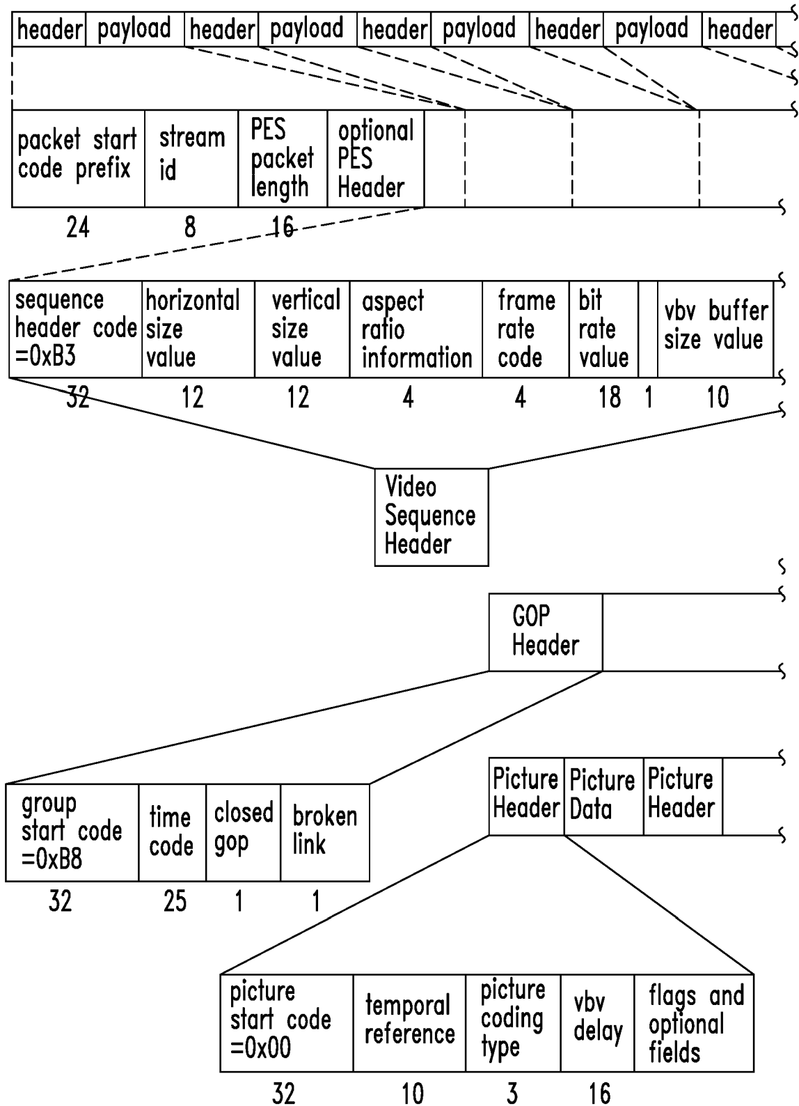
Figure 12 Parsing for bit_rate_value and stream_id
