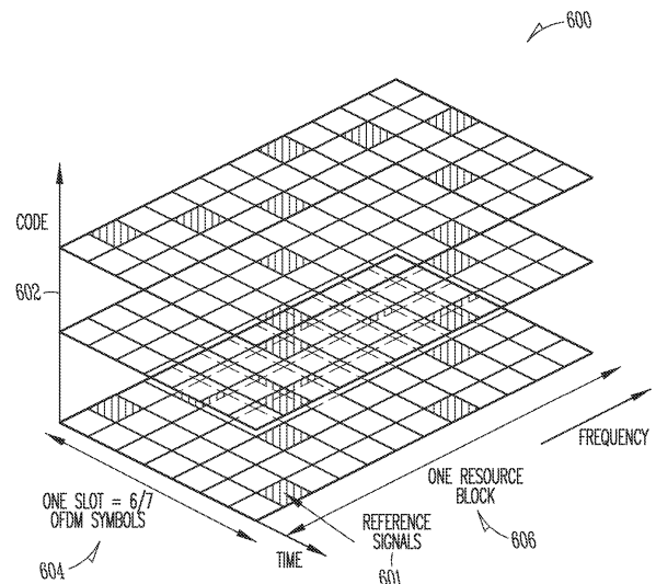
REFERENCE SIGNAL MULTIPLEXING SCHEME FIG. 6
