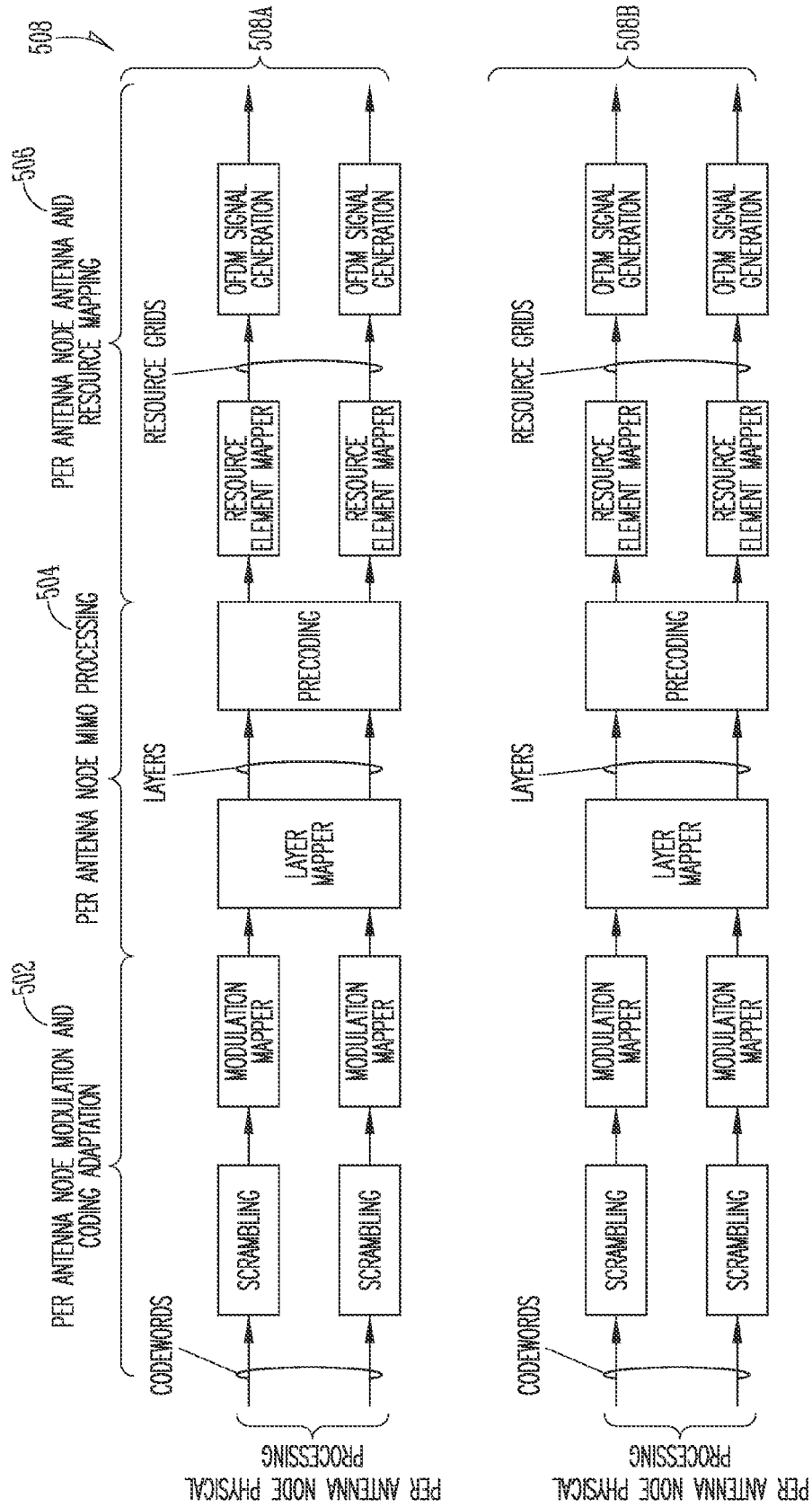
ANTENNA NODE PHY-LAYER PROCESSING
