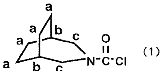
Chemical Formula 5
