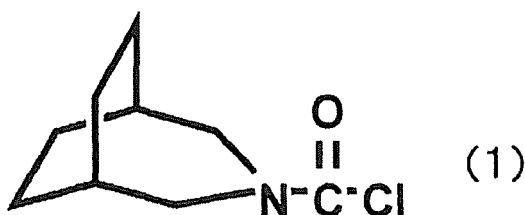
[Chemical Formula 2]
