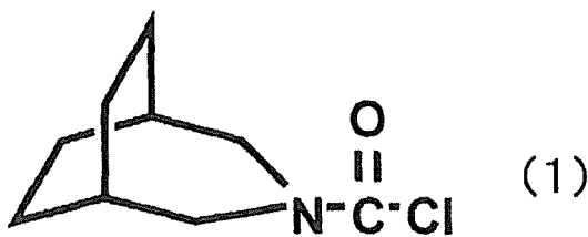
[Chemical Formula 3]
