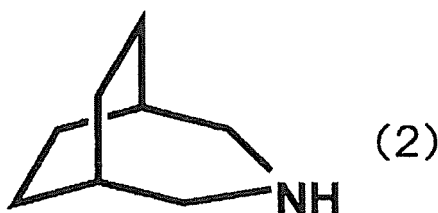
[Chemical Formula 4]
