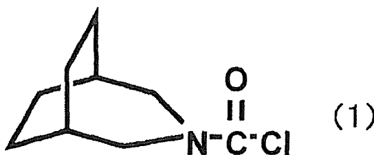
[Chemical Formula 3]
