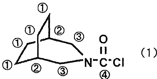
Chemical Formula 6
