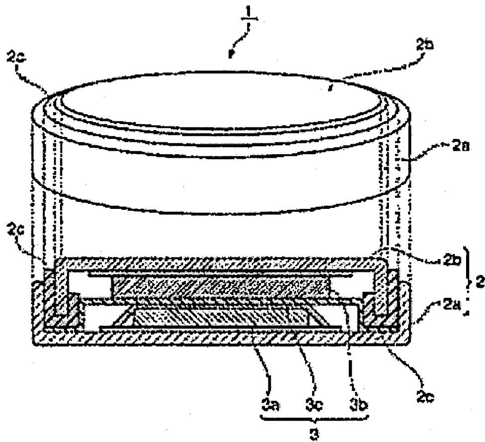
2032-type coin battery
