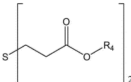
[Chemical Formula 7]
