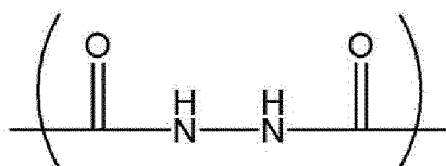
[Chemical Formula 8]
