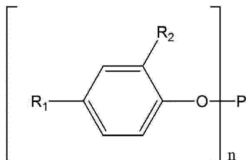
[Chemical Formula 4]
