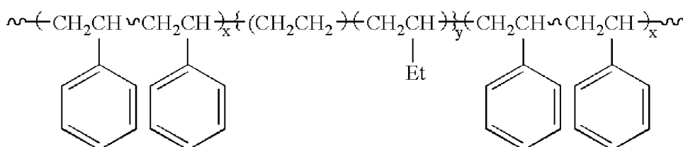
[Chemical Formula 11]
