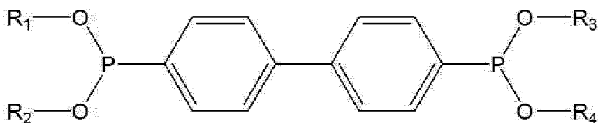
[Chemical Formula 5]
