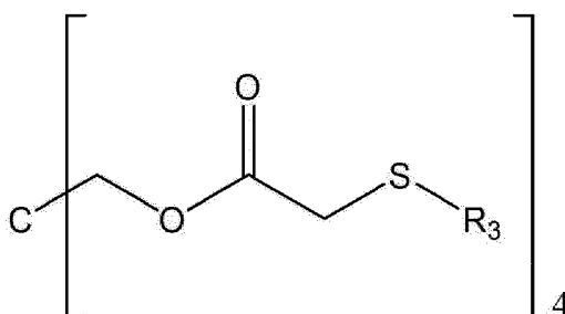
[Chemical Formula 7]
