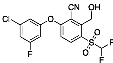
6-(3-Chloro-5-fluorophenoxy)-3-((difluoromethyl)sulfonyl)-2-(hydroxymethyl)benzonitrile ( Compound 35 )
