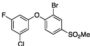
2-Bromo-1-(3-chloro-5-fluorophenoxy)-4-(methylsulfonyl)benzene ( Compound 138 )
