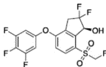
Compound 188
