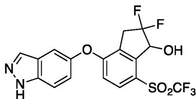
4-((1 H -Indazol-5-yl)oxy)-2,2-difluoro-7-((trifluoromethyl)sulfonyl)-2,3-dihydro-1 H -inden-1-ol ( Compound 238 )
