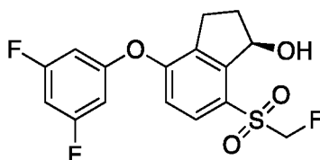
( R )-4-(3,5-Difluorophenoxy)-7-((fluoromethyl)sulfonyl)-2,3-dihydro-1 H -inden-1-ol ( Compound 60 )
