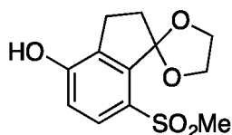
7-(Methylsulfonyl)-2,3-dihydrospiro[indene-1,2'-[1,3]dioxolan]-4-ol
