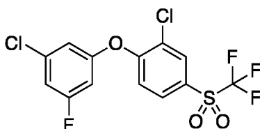
2-Chloro-1-(3-chloro-5-fluorophenoxy)-4-((trifluoromethyl)sulfonyl)benzene ( Compound 128 )
