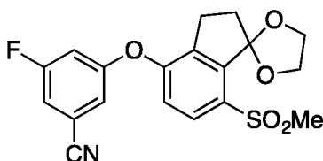
3-Fluoro-5-((7-(methylsulfonyl)-2,3-dihydrospiro[indene-1,2'-[1,3]dioxolan]-4-yl)oxy)benzonitrile
