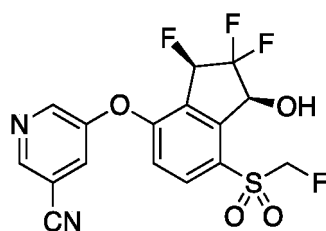
Compound 344
