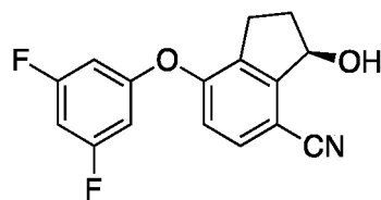
( R )-7-(3,5-Difluorophenoxy)-3-hydroxy-2,3-dihydro-1 H -indene-4-carbonitrile ( Compound 66 )
