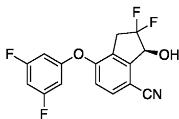
( S )-7-(3,5-Difluorophenoxy)-2,2-difluoro-3-hydroxy-2,3-dihydro-1 H -indene-4-carbonitrile ( Compound 67 )
