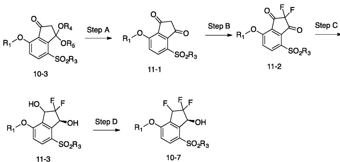
Scheme 11
