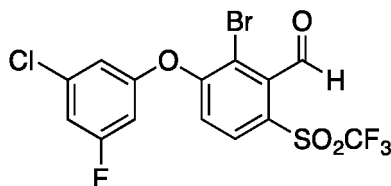
2-Bromo-3-(3-chloro-5-fluorophenoxy)-6-((trifluoromethyl)sulfonyl)benzaldehyde ( Compound 101 )
