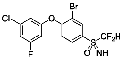
2-bromo-1-(3-chloro-5-fluorophenoxy)-4-((difluoromethyl)sulfonimidoyl)benzene ( Compound 69 )
