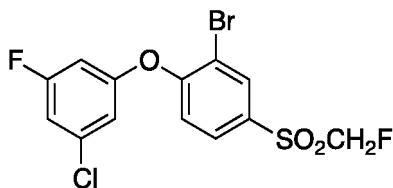
2-Bromo-1-(3-chloro-5-fluorophenoxy)-4-((fluoromethyl)sulfonyl)benzene ( Compound 137 )
