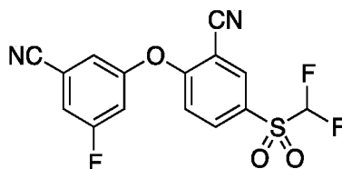
2-(3-Cyano-5-fluorophenoxy)-5-((difluoromethyl)sulfonyl)benzonitrile ( Compound 134 )
