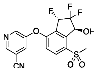
Compound 343
