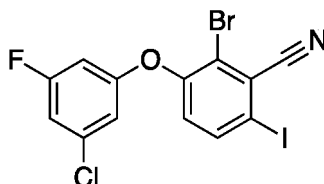
2-Bromo-3-(3-chloro-5-fluorophenoxy)-6-iodobenzonitrile ( Compound 96 )
