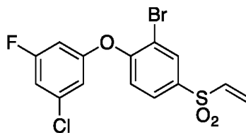
2-Bromo-1-(3-chloro-5-fluorophenoxy)-4-(vinylsulfonyl)benzene ( Compound 130 )
