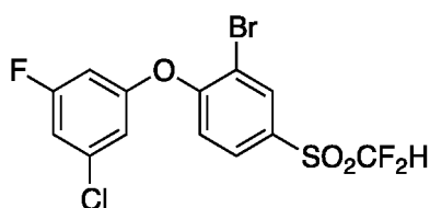
2-Bromo-1-(3-chloro-5-fluorophenoxy)-4-((difluoromethyl)sulfonyl)benzene ( Compound 131 )
