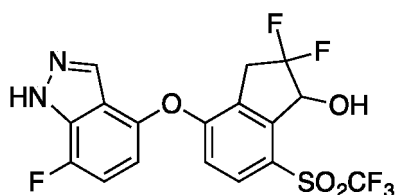
2,2-Difluoro-4-((7-fluoro-1 H -indazol-4-yl)oxy)-7-((trifluoromethyl)sulfonyl)-2,3-dihydro-1 H -inden-1-ol ( Compound 241 )
