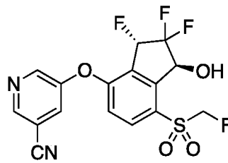
Compound 345
