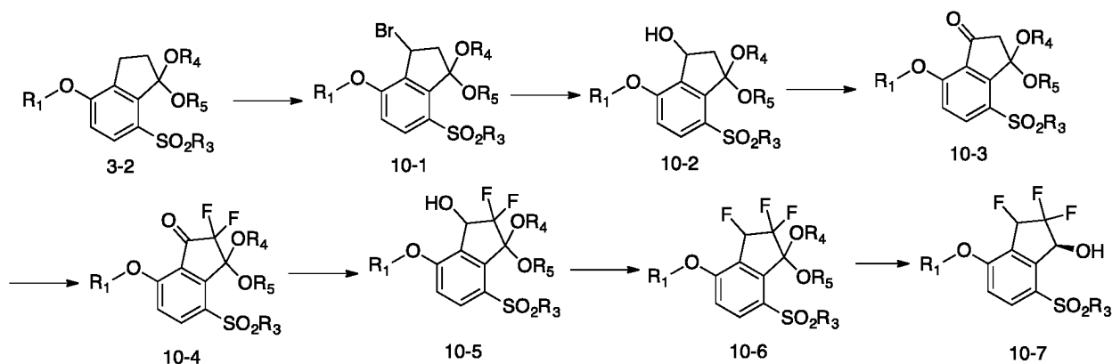
Scheme 10
