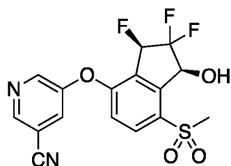
Compound 342
