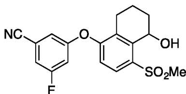
3-Fluoro-5-((5-hydroxy-4-(methylsulfonyl)-5,6,7,8-tetrahydronaphthalen-1-yl)oxy)benzonitrile ( Compound 95 )
