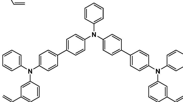
Hole transport compound 4
