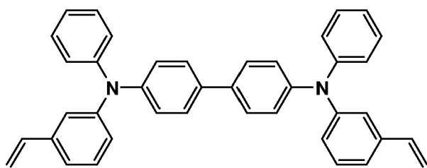
Hole transport compound 1
