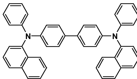
Hole transport compound 2
