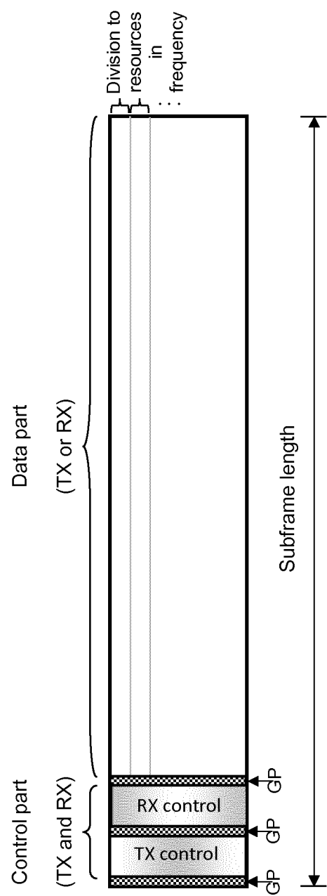
FIG. 12 (PRIOR ART)
