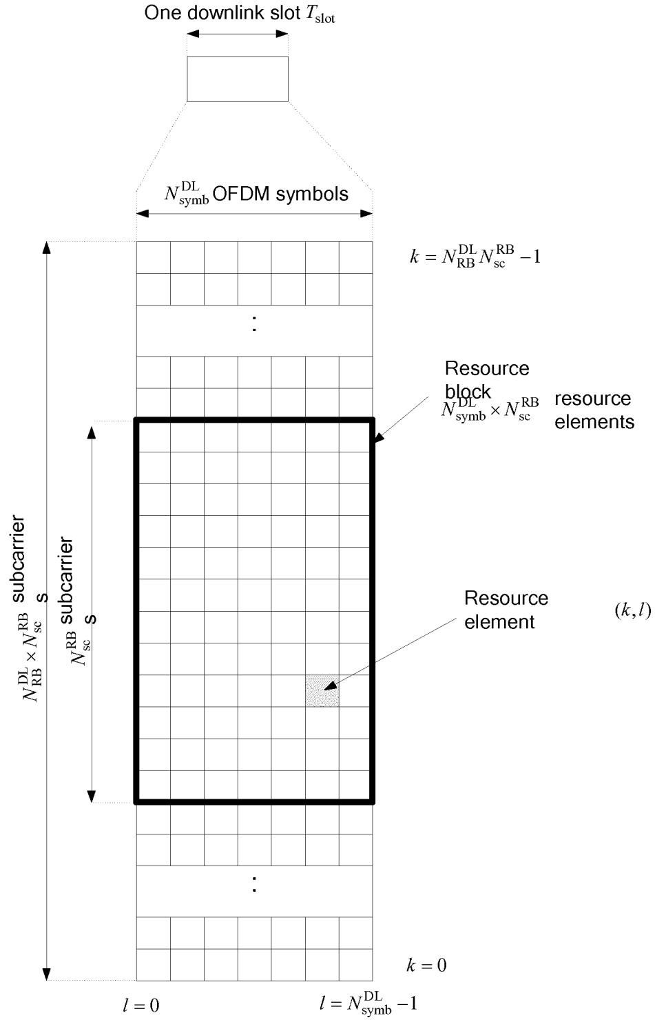
FIG. 10 (PRIOR ART)
