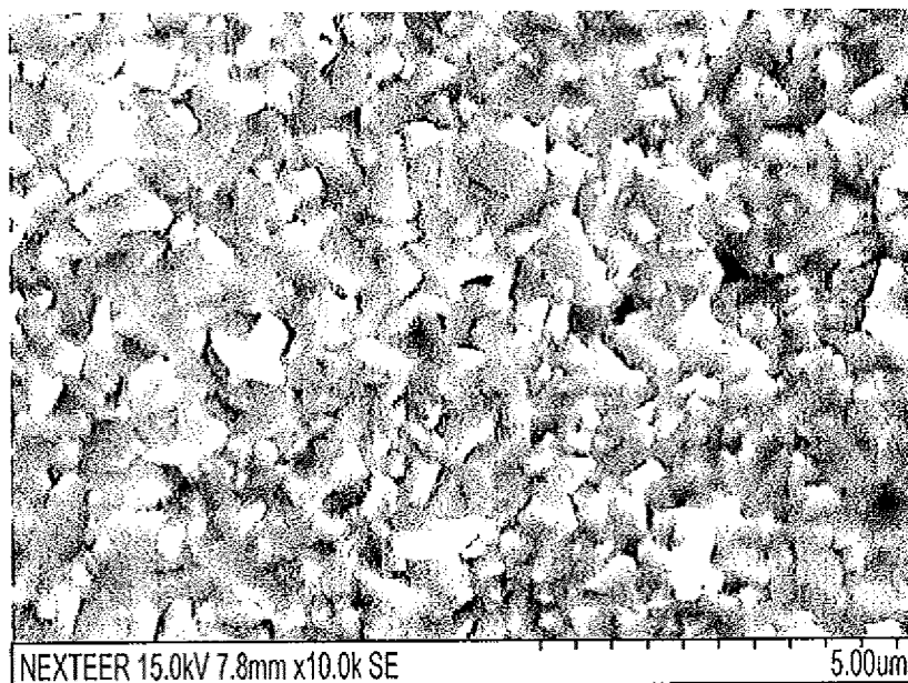
SURFACE OF STEAM TREATED PM HUB @ 10,000X
