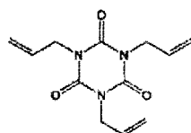
[Chem. 33]
