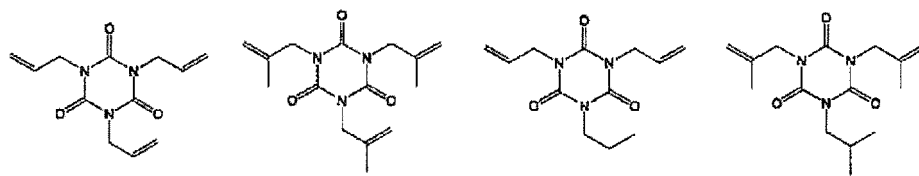
[Chem. 32]
