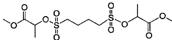
1-Methoxycarbonyl ethyl 1,4-butanedisulfonate
