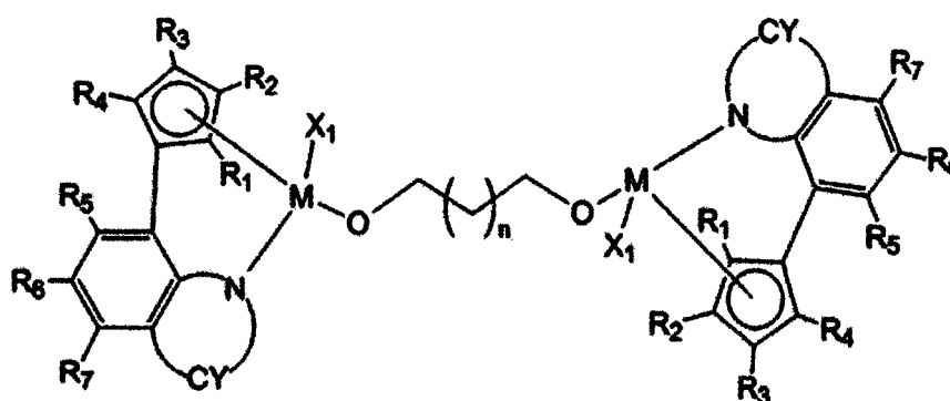
[Chemical Formula 1]
