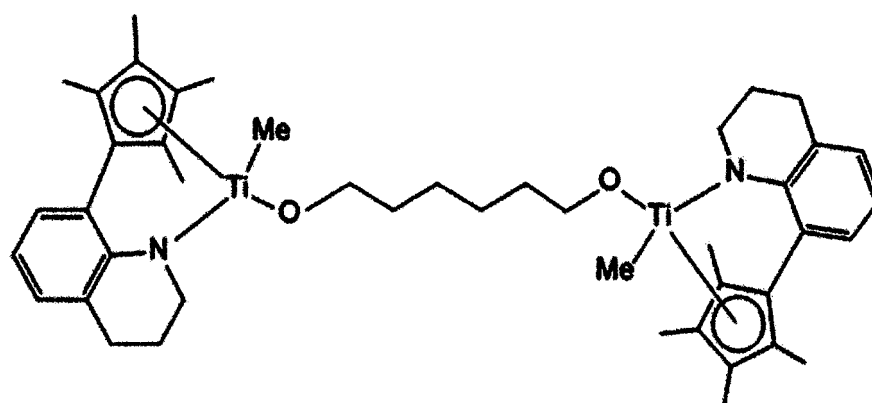
[Chemical Formula 9]
