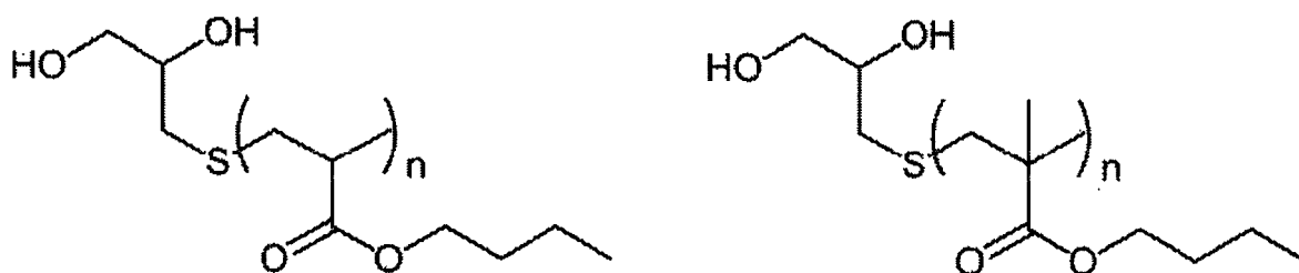
PMMA/PBMA-OH2 (Mn=6,000) m/n=50/50 (mass%)
