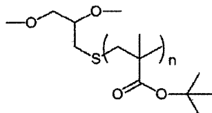
PtBMA-OH2 (Mn=5,000)
