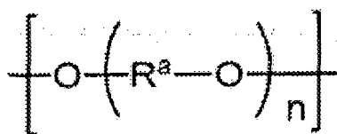
Formel (C)
