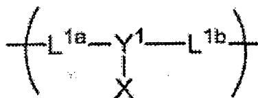
Formel (A)
