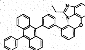
[Chemical Formula 1-8-17]
