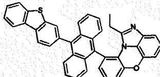
[Chemical Formula 1-8-13]
