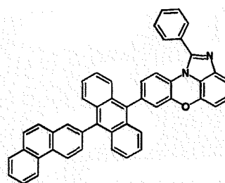
[Chemical Formula 1-4-6]
