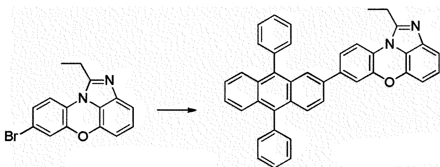
[Compound 2-A]
