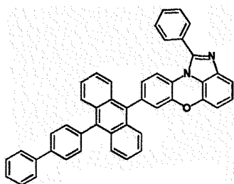
[Chemical Formula 1-4-4]
