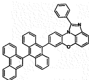
[Chemical Formula 1-4-7]
