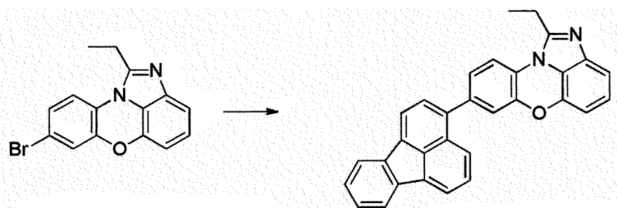
[Compound 2-A]
