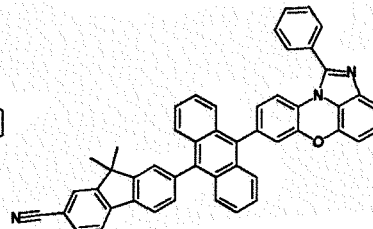
[Chemical Formula 1-4-14]
