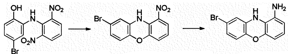
[Compound 17-A]
