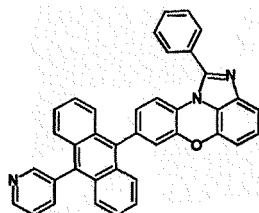
[Chemical Formula 1-4-10]
