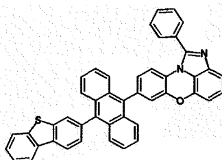
[Chemical Formula 1-4-13]
