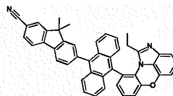
[Chemical Formula 1-8-14]
