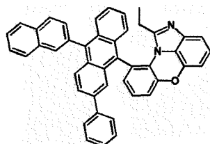
[Chemical Formula 1-8-16]
