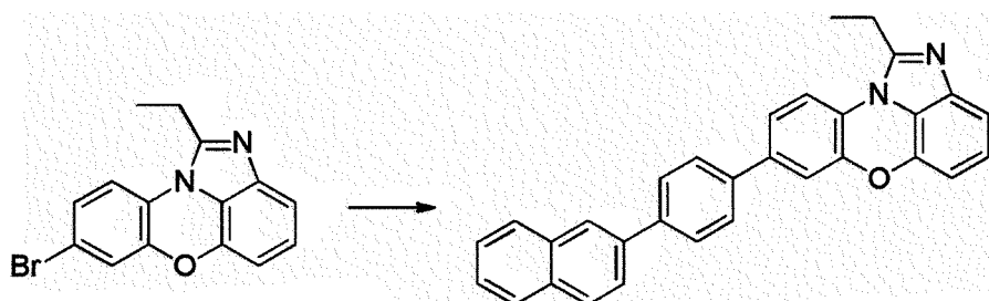
[Compound 2-A]
