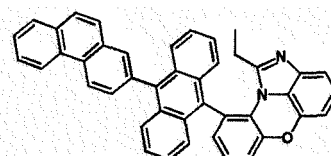
[Chemical Formula 1-8-8]
