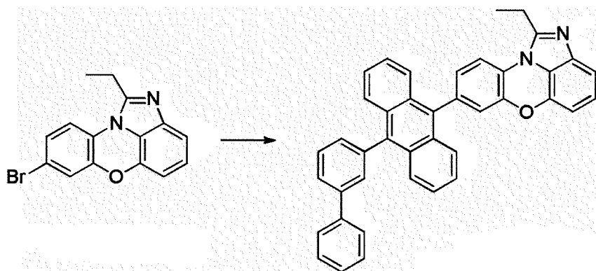
[Compound 2-A]
