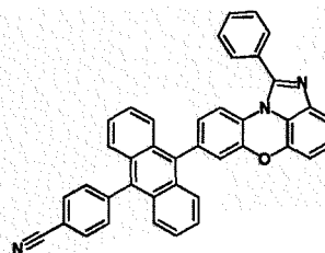
[Chemical Formula 1-4-11]
