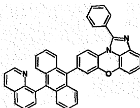
[Chemical Formula 1-4-10]
