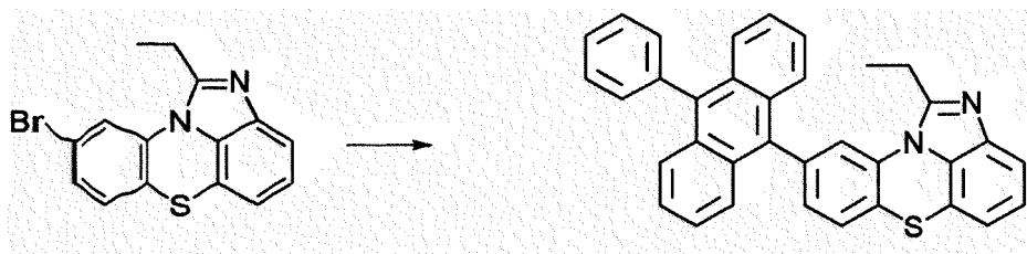
[Compound 2-2-D]
