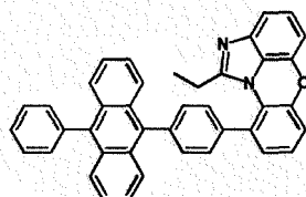
[Chemical Formula 1-8-16]
