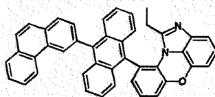
[Chemical Formula 1-8-8]
