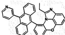
[Chemical Formula 1-8-10]
