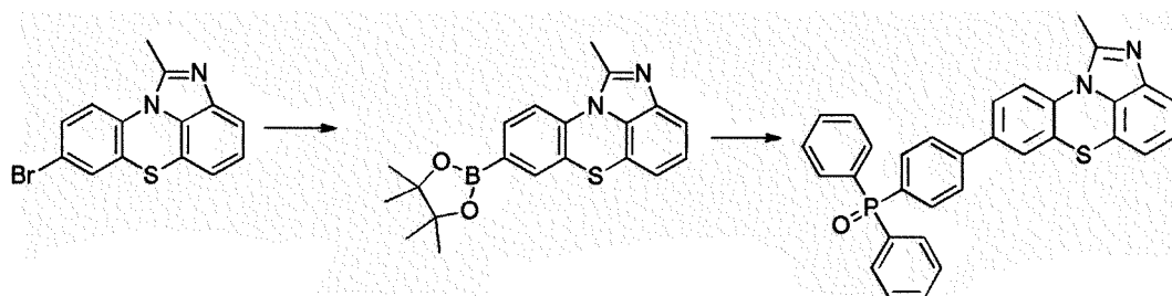
[Compound 2-1-D]
