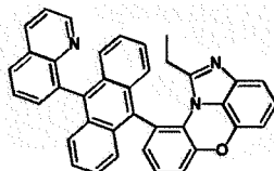
[Chemical Formula 1-8-10]
