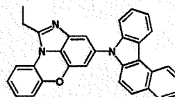
[Chemical Formula 1-10-13] [Chemical Formula 1-10-14] [Chemical Formula 1-10-15]
