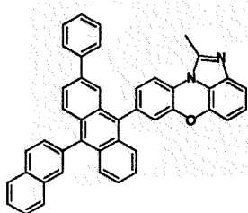
[Chemical Formula 1-2-16] [Chemical Formula 1-2-17] [Chemical Formula 1-2-18]
