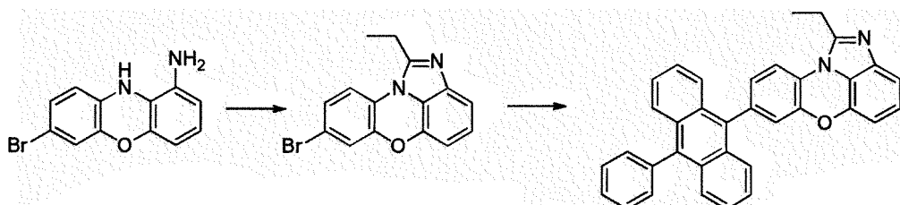
[Compound 1-C]
