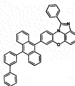
[Chemical Formula 1-4-5]
