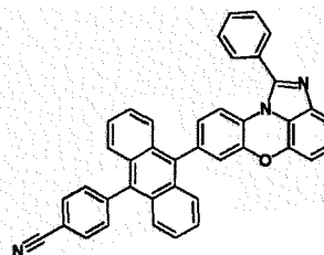
[Chemical Formula 1-4-11]
