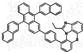
[Chemical Formula 2-3-25] [Chemical Formula 2-3-26] [Chemical Formula 2-3-27]
