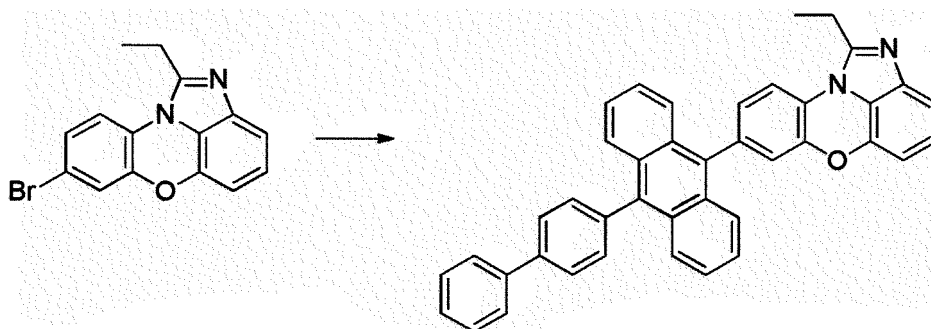
[Compound 2-A]
