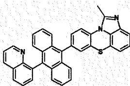
[Chemical Formula 2-2-10] [Chemical Formula 2-2-11] [Chemical Formula 2-2-12]
