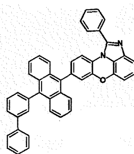
[Chemical Formula 1-4-5]
