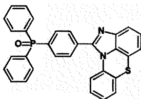
[Chemical Formula 2-1-9] [Chemical Formula 2-1-10].
