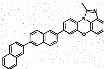
[Chemical Formula 1-2-43] [Chemical Formula 1-2-44] [Chemical Formula 1-2-45]
