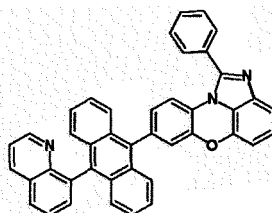
[Chemical Formula 1-4-10]
