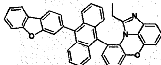
[Chemical Formula 1-8-13]
