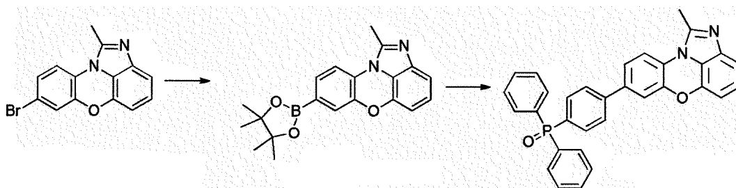
[Compound 1-D]
