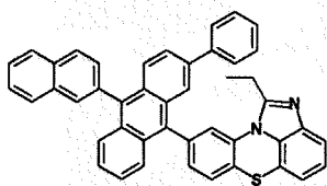
[Chemical Formula 2-3-16] [Chemical Formula 2-3-17] [Chemical Formula 2-3-18]
