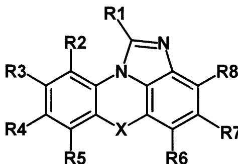
[Chemical Formula 1]
