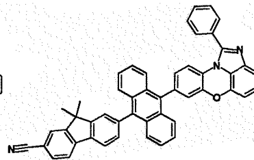
[Chemical Formula 1-4-14]
