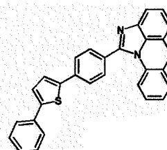
[Chemical Formula 1-1-45] [Chemical Formula 1-1-46] [Chemical Formula 1-1-47]
