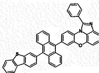
[Chemical Formula 1-4-13]
