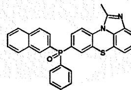
[Chemical Formula 2-4-1] [Chemical Formula 2-4-2] [Chemical Formula 2-4-3]
