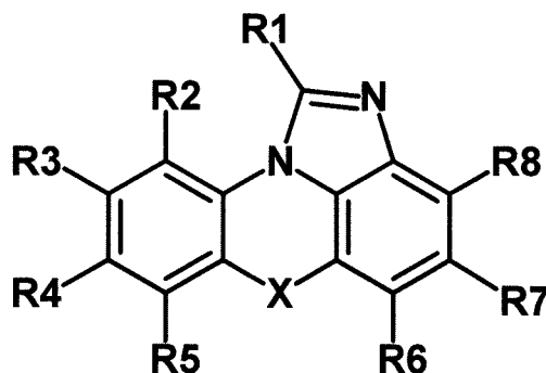
[Chemical Formula 3]
