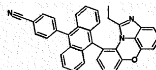
[Chemical Formula 1-8-11]
