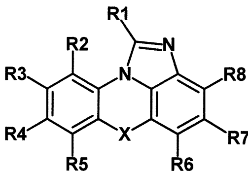
[Chemical Formula 3]
