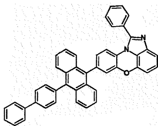
[Chemical Formula 1-4-4]
