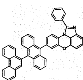
[Chemical Formula 1-4-7]
