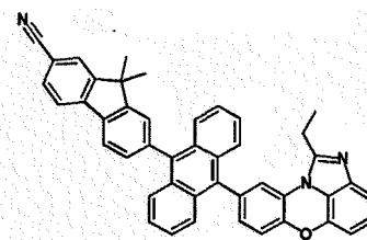
[Chemical Formula 1-7-10] [Chemical Formula 1-7-11] [Chemical Formula 1-7-12]
