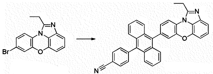
[Compound 2-A]
