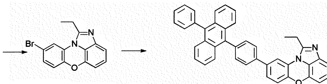
[Compound 17-D]
