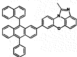
[Chemical Formula 1-2-22] [Chemical Formula 1-2-23] [Chemical Formula 1-2-24]
