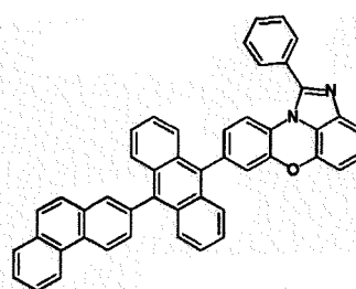
[Chemical
