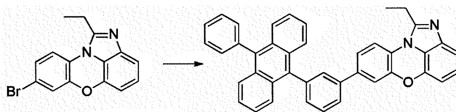
[Compound 2-A]
