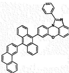
[Chemical Formula 1-4-7]
