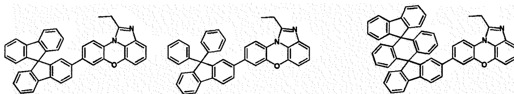
[Chemical Formula 1-3-34] [Chemical Formula 1-3-35] [Chemical Formula 1-3-36]
