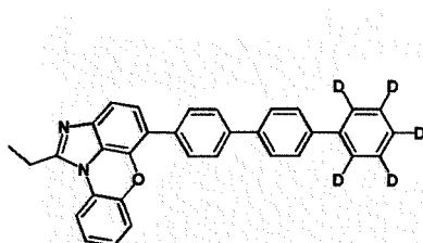
[Chemical Formula 1-9-16] [Chemical Formula 1-9-17] [Chemical Formula 1-9-18]
