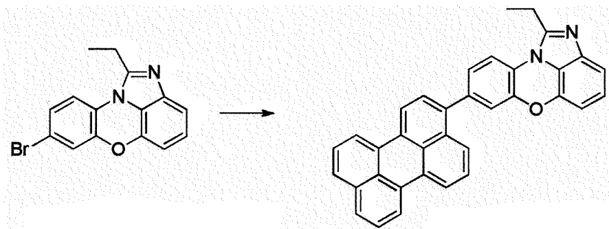
[Compound 2-A]
