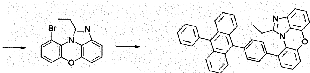
[Compound 18-D]
