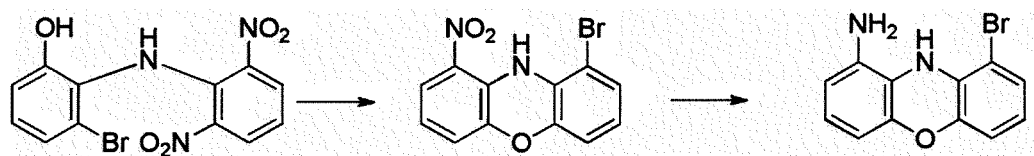
[Compound 18-A]
