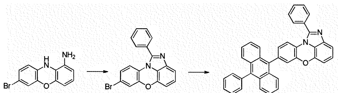
[Compound 1-C]
