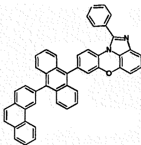
[Chemical Formula 1-4-8]
