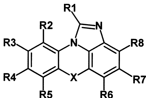
[Chemical Formula 3]
