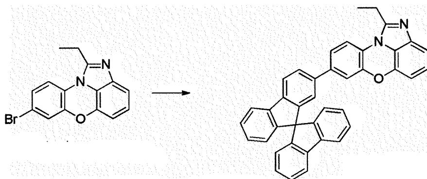
[Compound 2-A]
