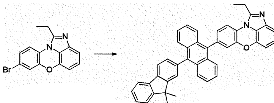
[Compound 2-A]
