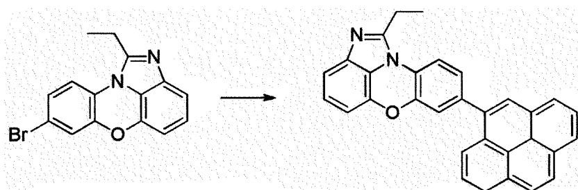
[Compound 2-A]
