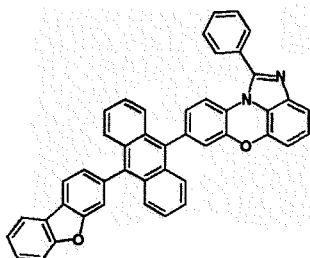
[Chemical Formula 1-4-13]
