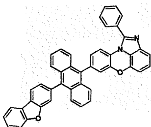
[Chemical Formula 1-4-13]
