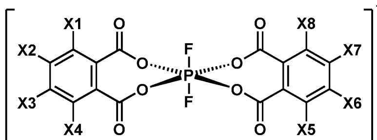
[Chemical Formula 2]
