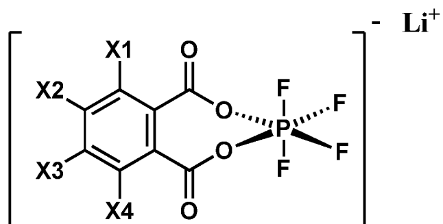
[Chemical Formula 1-1]
