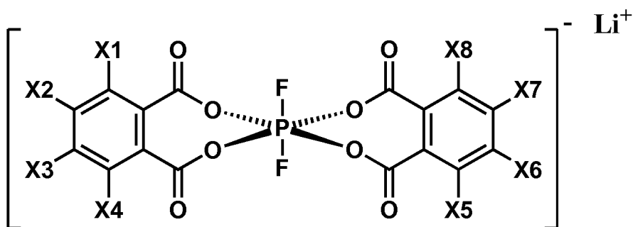
[Chemical Formula 3-1]
