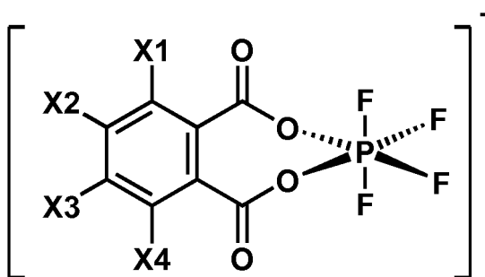
[Chemical Formula 1]
