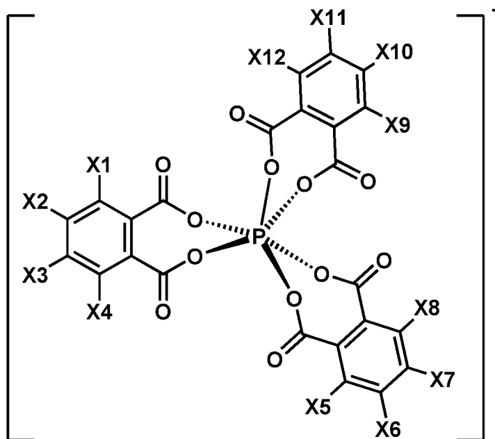
[Chemical Formula 3]
