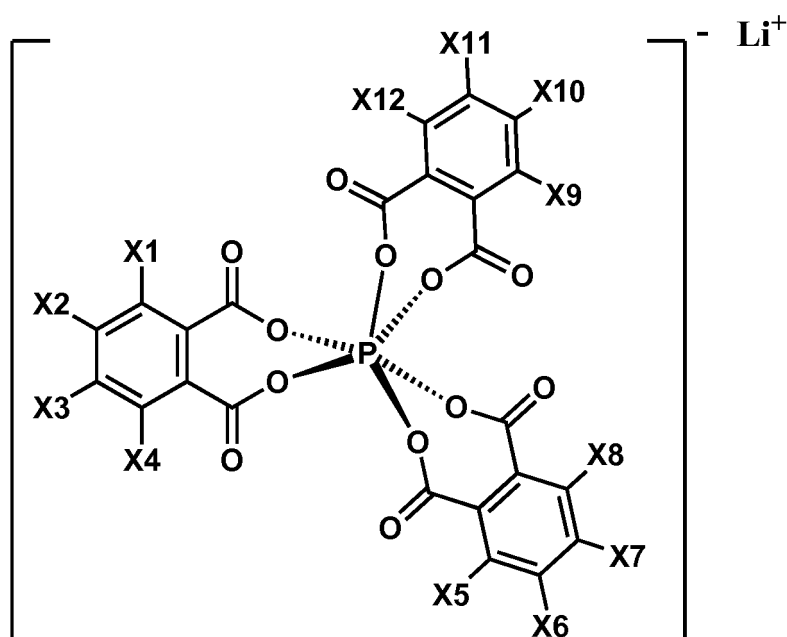
[Chemical Formula 3-1]
