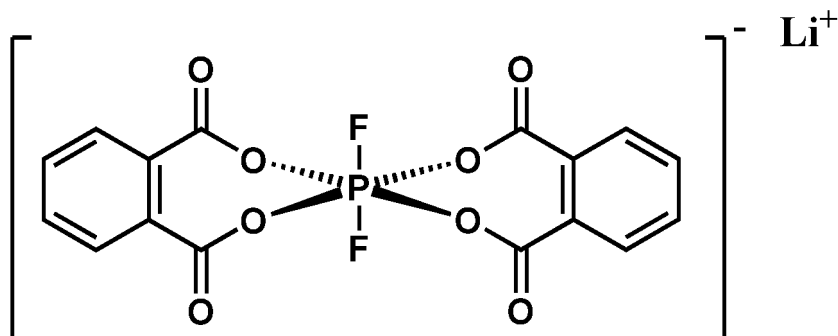
[Chemical Formula 2-2]
