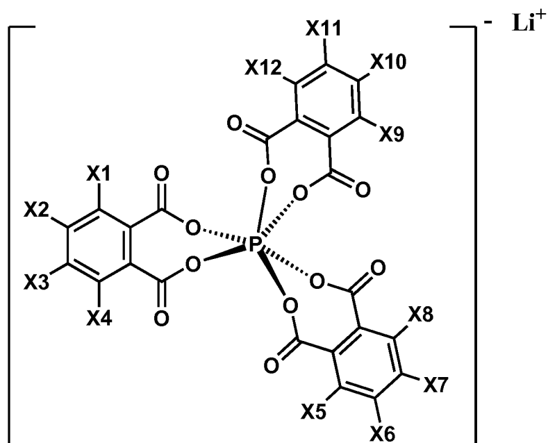
[Chemical Formula 3-1]
