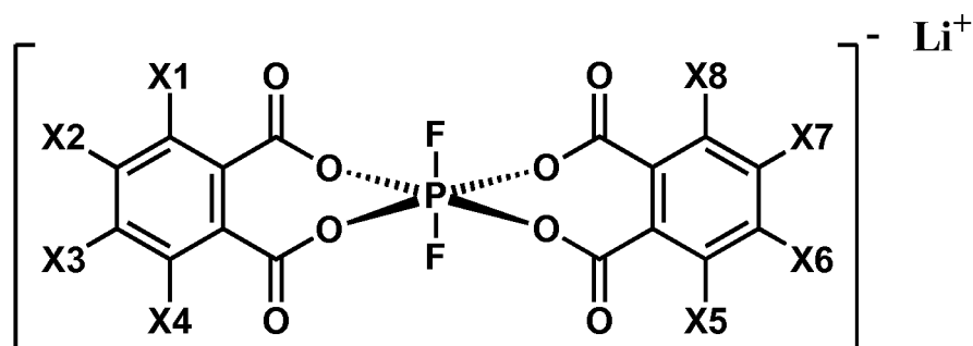
[Chemical Formula 2-1]
