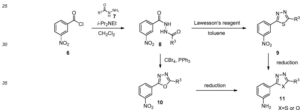
Scheme 2
