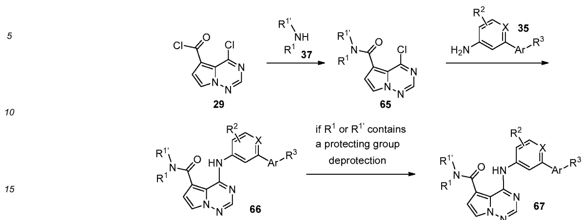
Scheme 16
