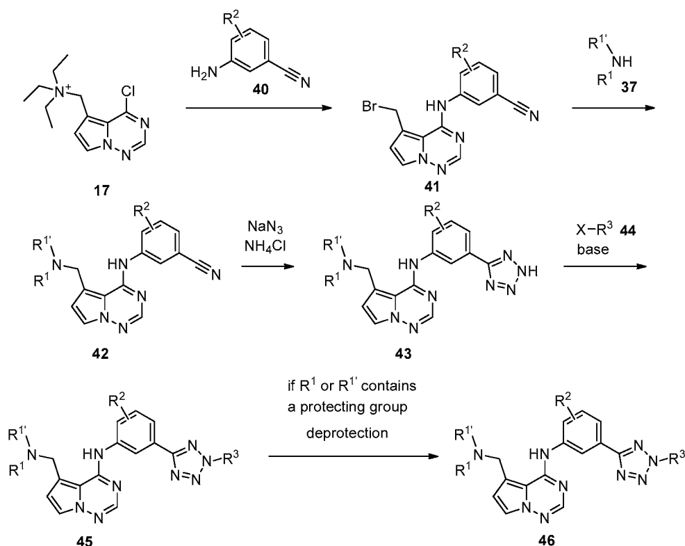
Scheme 10
