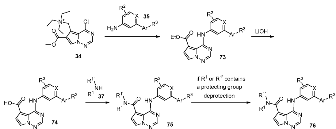
Scheme 18
