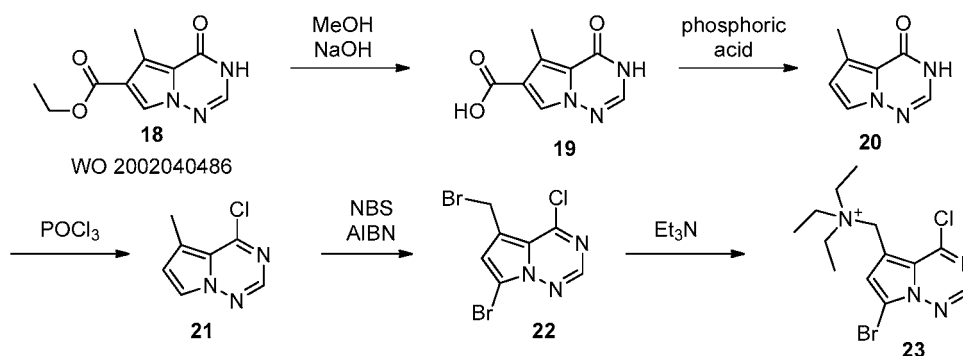
Scheme 5
