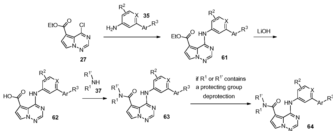
Scheme 15
