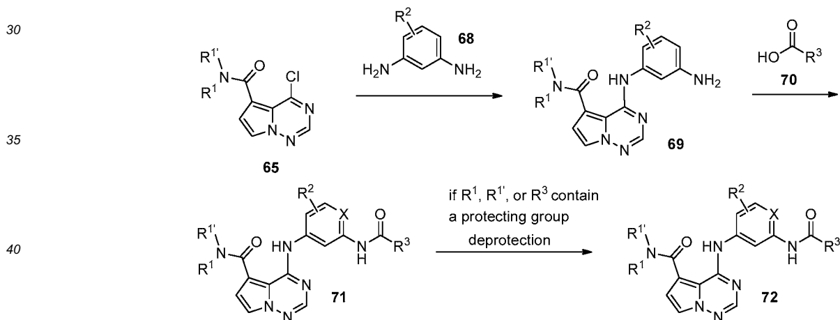
Scheme 17
