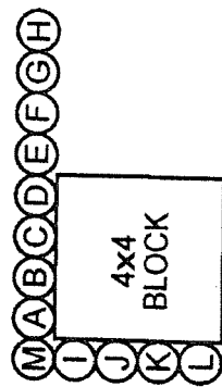
(a) Intra_4x4
