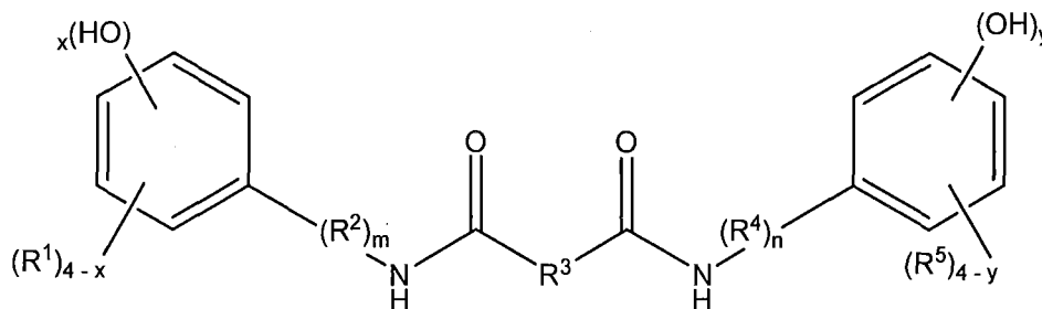
Formula II
