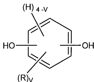
Formula E
