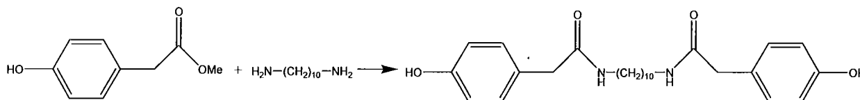
Formula IA
