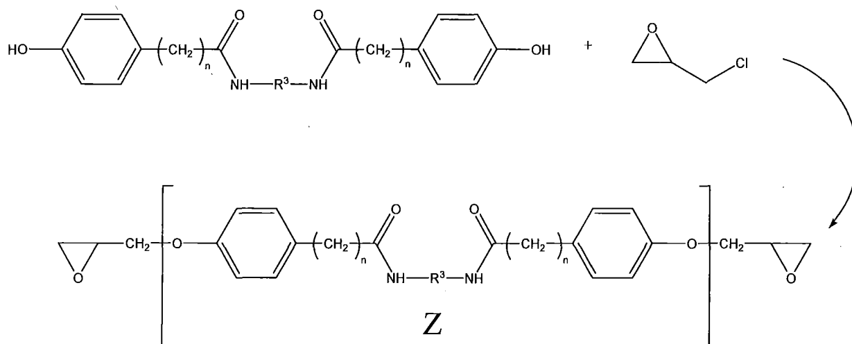
Formula VIII
