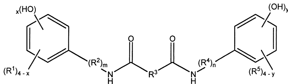
Formel (II),
