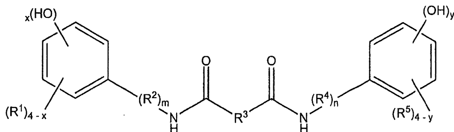
Formula II
