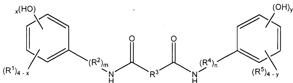
Formula (II),
