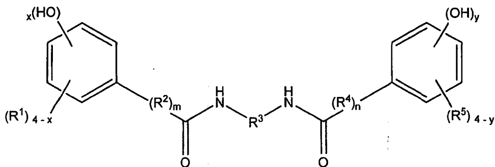
Formula I
