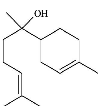
bisabolol (CAS # 515-69-5)
