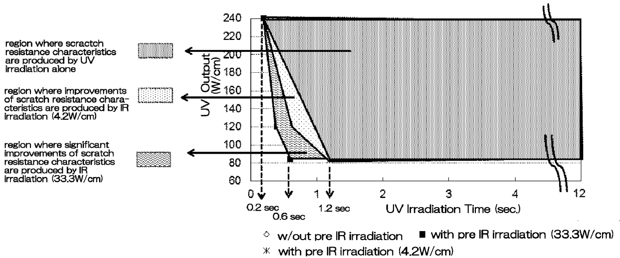
UV Irradiation Time and Output for Producing Excellence of Resistance Against SW by IR Irradiation
