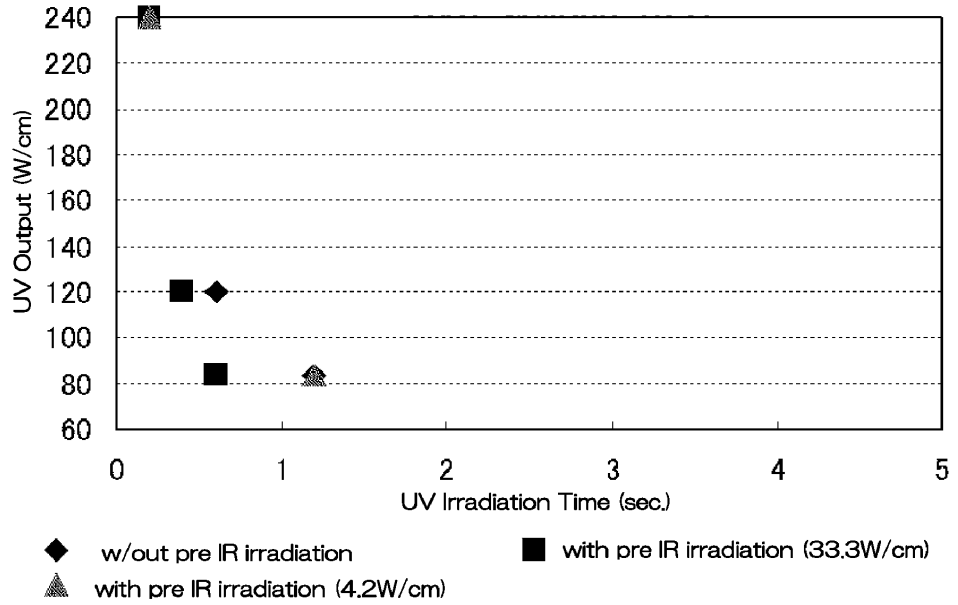
UV Irradiation Time and Output for Producing Excellence of Resistance Against SW by IR Irradiation
