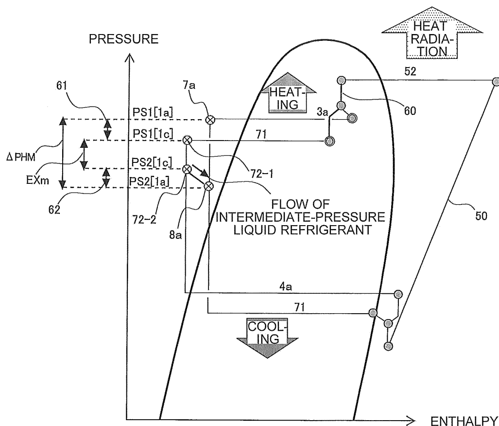
P-H DIAGRAM IN COOLING MAIN OPERATION MODE
