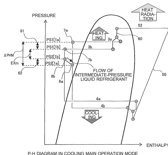
P-H DIAGRAM IN COOLING MAIN OPERATION MODE
