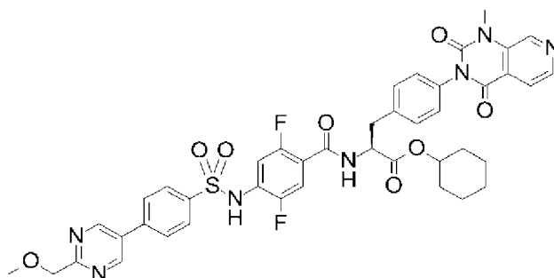
(g) (2S)-2-[[2,5-difluoro-4-[[4-[2-(methoxymethyl)pyrimidin-5-yl]phenyl]sulfonylamino]benzoyl]amino]-3-[4-(1-methyl-2,4-dioxo-pyrido[3,4-d]pyrimidin-3-yl)phenyl]propanoate
