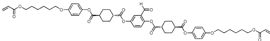
Intermediate C
