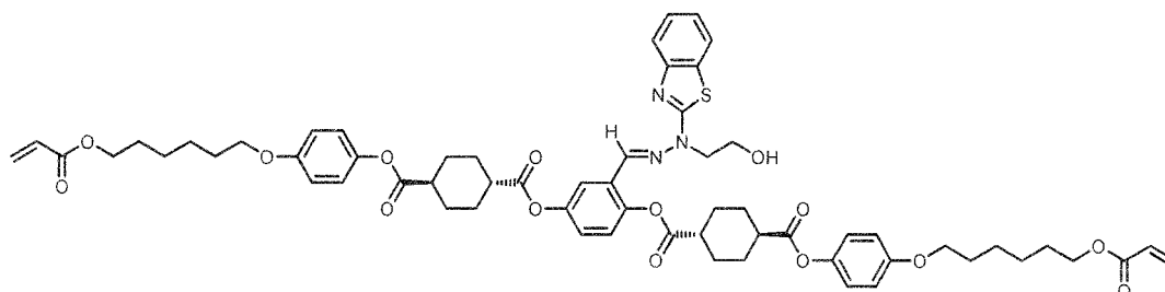
Intermediate D
