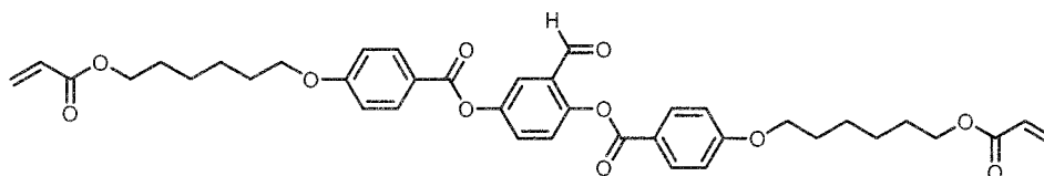
Intermediate E
