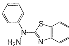
Intermediate α
