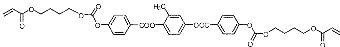
Compound 2r
