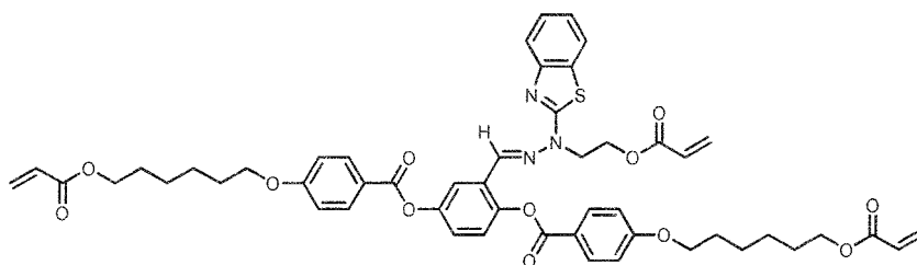
Compound 2
