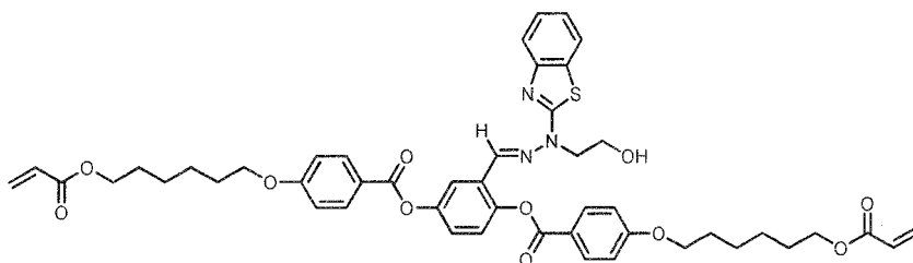
Intermediate F
