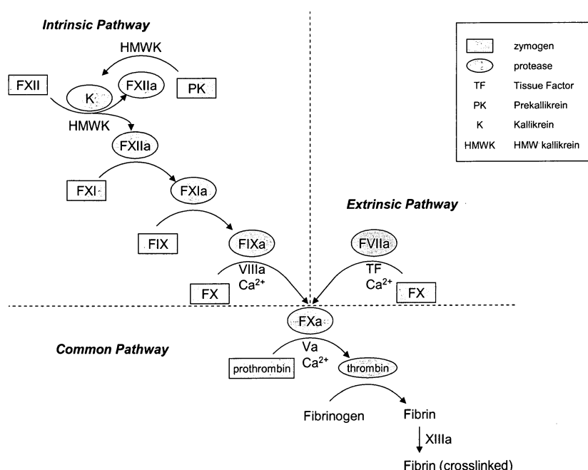
Figure 1. Coagulation cascade
