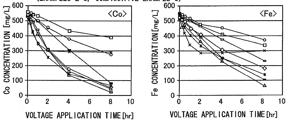
Fig.8 ELECTRODEPOSITION TEST RESULTS (EXAMPLES 2-8, COMPARATIVE EXAMPLE 8)
