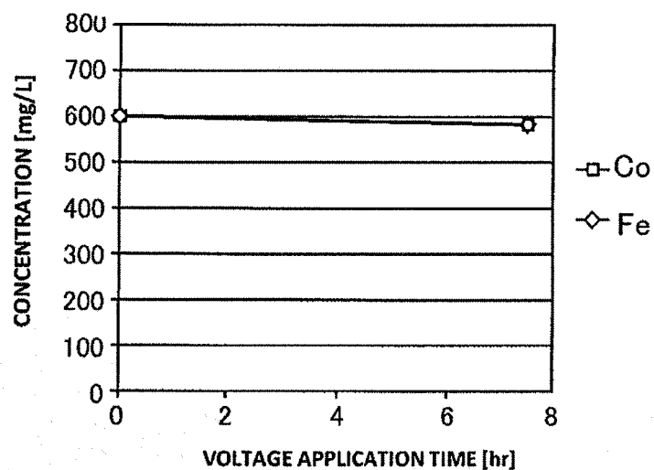
Fig.24 ELECTRODEPOSITION TEST RESULTS (COMPARATIVE EXPERIMENTAL EXAMPLE 2, EDTA)
