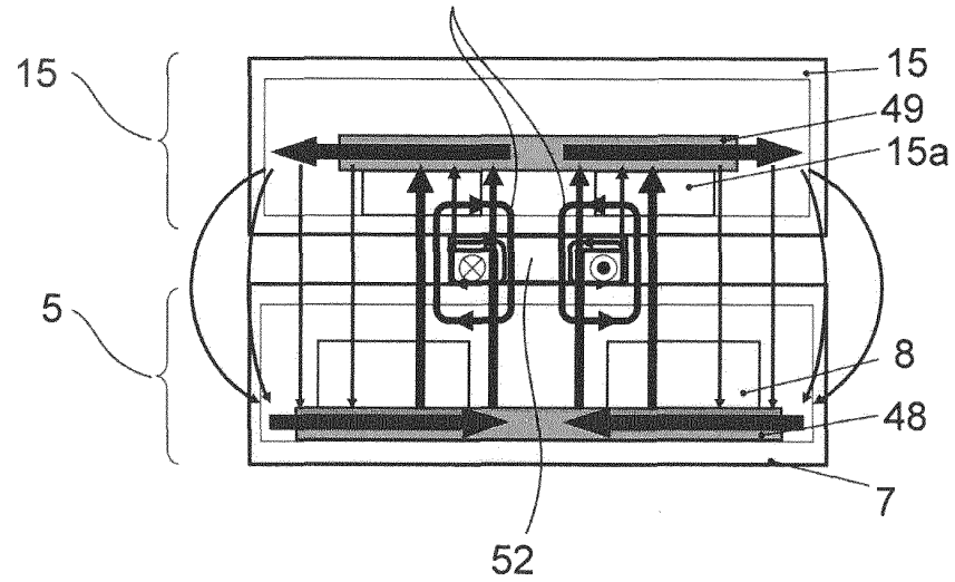
Magnetic flux line caused by eddy current
