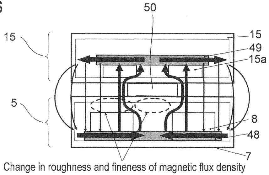
Magnetic flux line caused by eddy current
