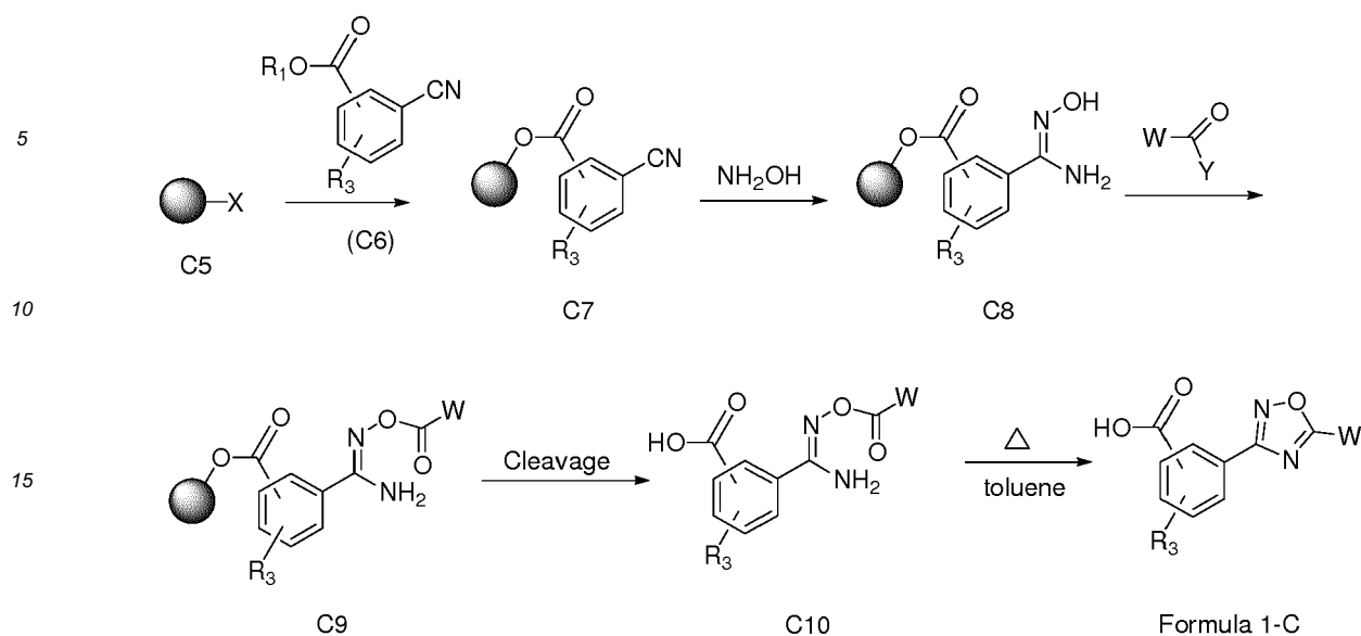
Scheme C2
