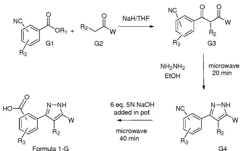
Scheme G1
