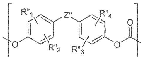
[Chemical Formula 6]
