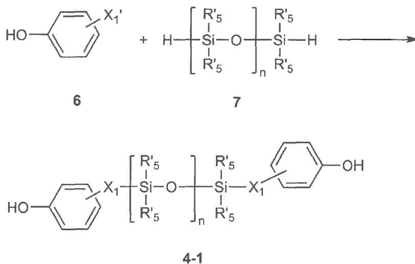
[Reaction Scheme 1]
