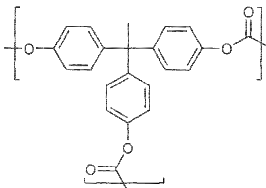
[Chemical Formula 2-2]
