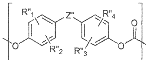
[Chemical Formula 6]
