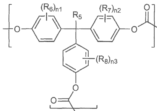
[Chemical Formula 2]
