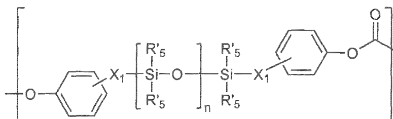
[Chemical Formula 4]
