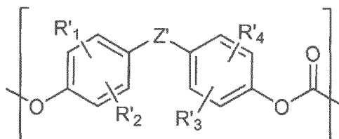
[Chemical Formula 3]
