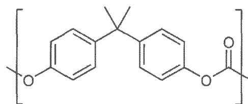
[Chemical Formula 3-1]
