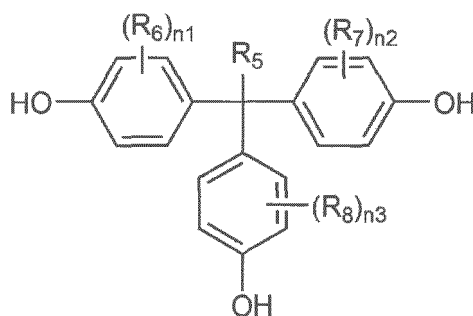
[Chemical Formula 2-1]
