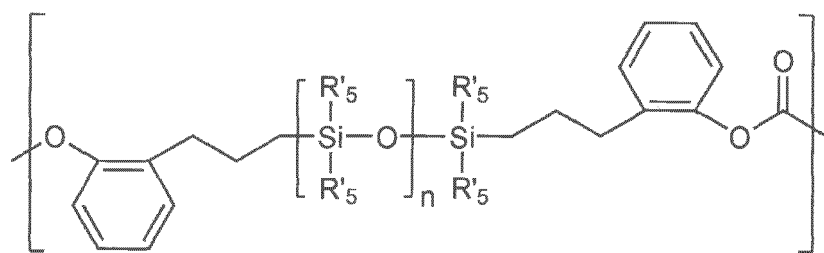
[Chemical Formula 4-2]
