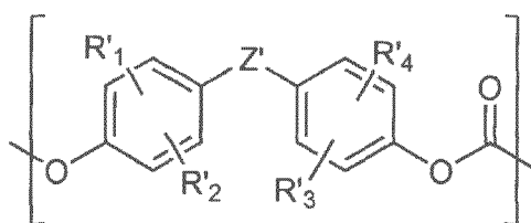
[Chemical Formula 3]
