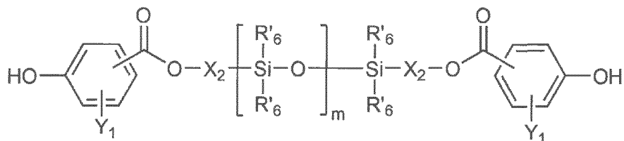
[Chemical Formula 5-1]
