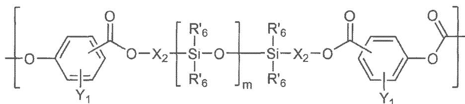
[Chemical Formula 5]
