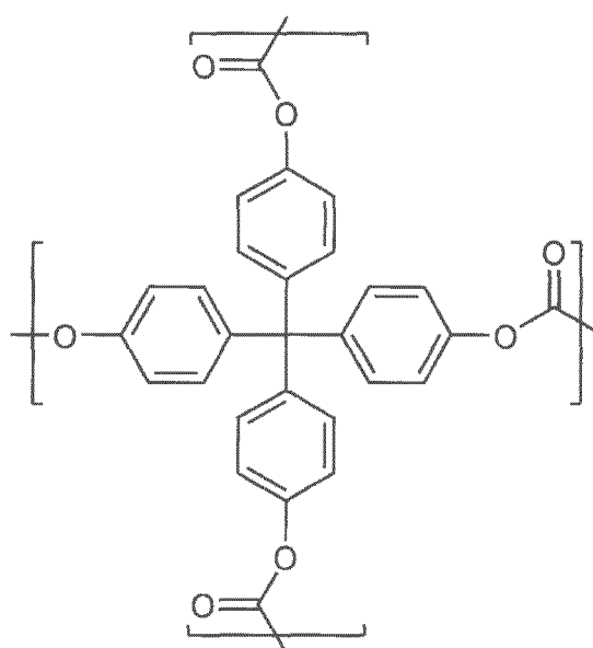
[Chemical Formula 2-3]
