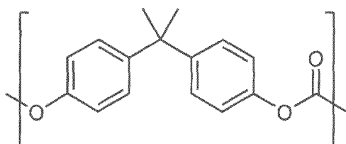
[Chemical Formula 3-1]
