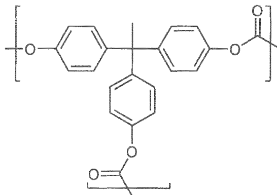
[Chemical Formula 2-2]
