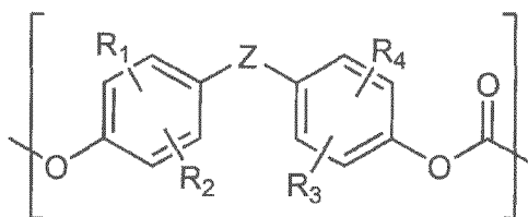
[Chemical Formula 1]
