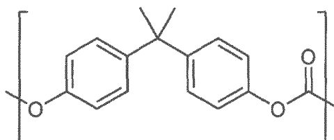
[Chemical Formula 6-1]
