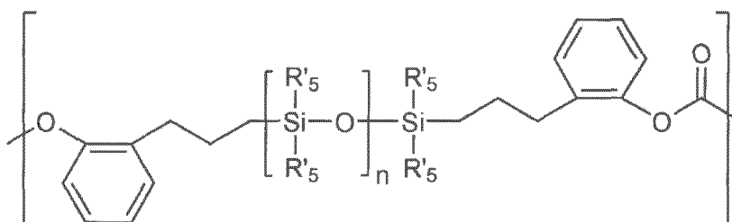
[Chemical Formula 4-2]
