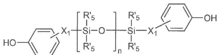
[Chemical Formula 4-1]
