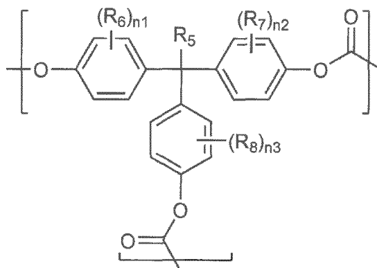
[Chemical Formula 2]
