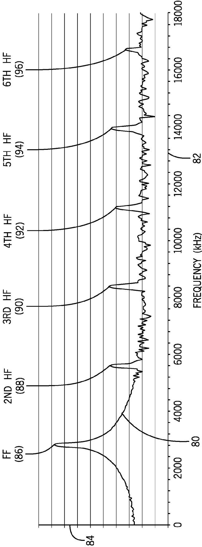
SPECTRUM PLOT OF KNOCK SENSOR DATA
