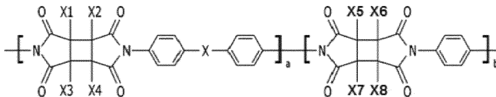
Chemical Formula 11
