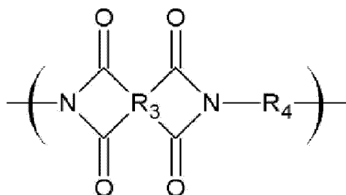
Chemical Formula 5
