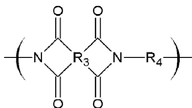
Chemical Formula 5
