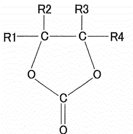
[Chem. 1]
