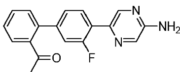
1-[4'-(5-Aminopyrazin-2-yl)-3'-fluorobiphenyl-2-yl]ethanone
