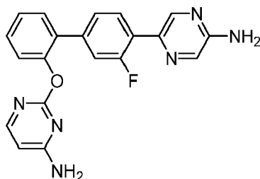
2-([4'-(5-Aminopyrazin-2-yl)-3'-fluorobiphenyl-2-yl]oxy)pyrimidin-4-amine
