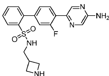
4'-(5-Aminopyrazin-2-yl)-N-(azetidin-3-ylmethyl)-3'-fluorobiphenyl-2-sulfonamide
