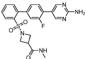
1-{[4'-(2-Aminopyrimidin-5-yl)-3'-fluorobiphenyl-2-yl]sulfonyl}-N-methylazetidine-3-carboxamide
