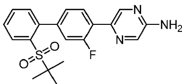
5-[2'-( tert -Butylsulfonyl)-3-fluorobiphenyl-4-yl]pyrazin-2-amine
