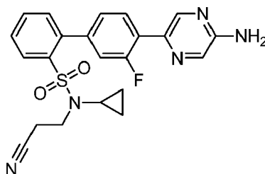
4'-(5-Aminopyrazin-2-yl)-N-(2-cyanoethyl)-N-cyclopropyl-3'-fluorobiphenyl-2-sulfonamide
