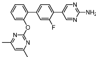
5-{2'-[(4,6-Dimethylpyrimidin-2-yl)oxy]-3-fluorobiphenyl-4-yl}pyrimidin-2-amine.
