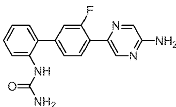
1-[4'-(5-Aminopyrazin-2-yl)-3'-fluorobiphenyl-2-yl]urea
