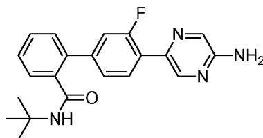
4'-(5-Aminopyrazin-2-yl)-N-tert-butyl-3'-fluorobiphenyl-2-carboxamide
