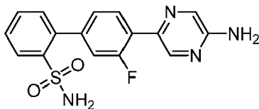
4'-(5-Aminopyrazin-2-yl)-3'-fluorobiphenyl-2-sulfonamide
