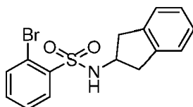
2-Bromo-N-(2,3-dihydro-1H-inden-2-yl)benzenesulfonamide
