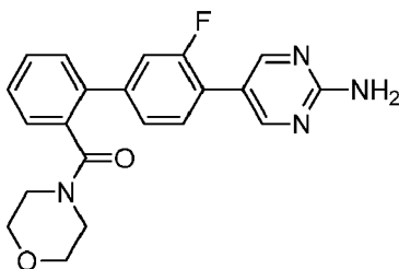
5-[3-Fluoro-2'-(morpholin-4-ylcarbonyl)biphenyl-4-yl]pyrimidin-2-amine
