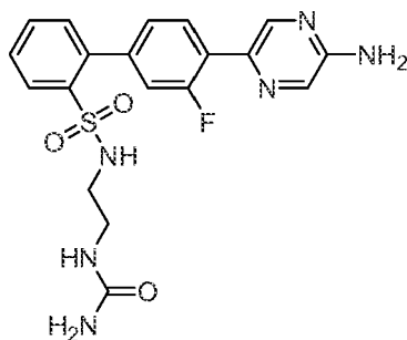
4'-(5-Aminopyrazin-2-yl)-N-[2-(carbamoylamino)ethyl]-3'-fluorobiphenyl-2-sulfonamide
