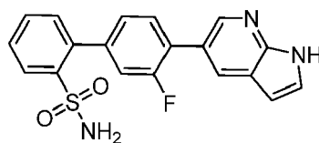
3'-Fluoro-4'-(1H-pyrrolo[2,3-b]pyridin-5-yl)biphenyl-2-sulfonamide
