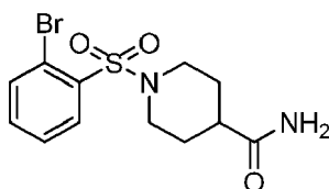
1-((2-Bromophenyl)sulfonyl)piperidine-4-carboxamide
