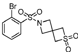
6-((2-Bromophenyl)sulfonyl)-2-thia-6-azaspiro[3.3]heptane 2,2-dioxide
