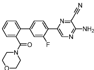
3-Amino-6-[3-fluoro-2'-(morpholin-4-ylcarbonyl)biphenyl-4-yl]pyrazine-2-carbonitrile
