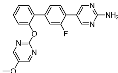
5-{3-Fluoro-2'-[(5-methoxypyrimidin-2-yl)oxy]biphenyl-4-yl}pyrimidin-2-amine
