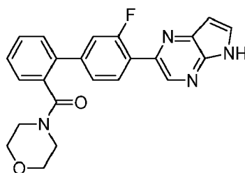
2-[3-Fluoro-2'-(morpholin-4-ylcarbonyl)biphenyl-4-yl]-5H-pyrrolo[2,3-b]pyrazine
