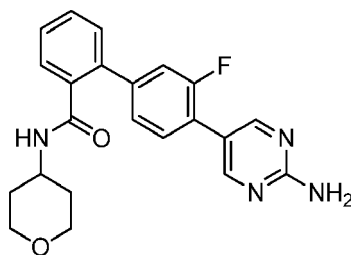
2-[4-(2-Aminopyrimidin-5-yl)-3-fluoro-phenyl]-N-tetrahydropyran-4-yl-benzamide
