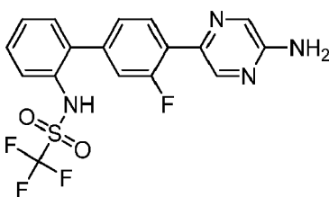
[4'-(5-Aminopyrazin-2-yl)-3'-fluorobiphenyl-2-yl]-1,1,1-trifluoromethanesulfonamide
