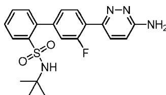
4'-(6-Aminopyridazin-3-yl)-N-tert-butyl-3'-fluorobiphenyl-2-sulfonamide
