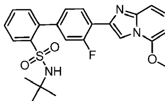
N-tert-Butyl-3'-fluoro-4'-(5-methoxyimidazo[1,2-a]pyridin-2-yl)biphenyl-2-sulfonamide
