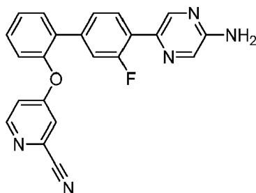
4-{[4'-(5-Aminopyrazin-2-yl)-3'-fluorobiphenyl-2-yl]oxy}pyridine-2-carbonitrile
