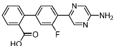
4'-(5-Aminopyrazin-2-yl)-3'-fluorobiphenyl-2-carboxylic acid
