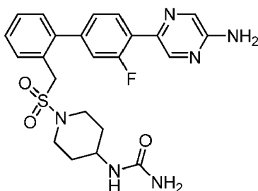
1-[1-({[4'-(5-Aminopyrazin-2-yl)-3'-fluorobiphenyl-2-yl]methyl}sulfonyl)piperidin-4-yl]urea hydrochloride
