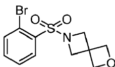
6-((2-Bromophenyl)sulfonyl)-2-oxa-6-azaspiro[3.3]heptane
