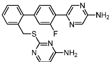
2-({[4'-(5-Aminopyrazin-2-yl)-3'-fluorobiphenyl-2-yl]methyl}sulfanyl)pyrimidin-4-amine
