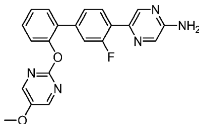
5-{3-Fluoro-2'-[(5-methoxypyrimidin-2-yl)oxy]biphenyl-4-yl}pyrazin-2-amine
