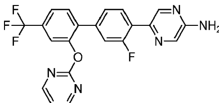
5-{3-Fluoro-2'-(pyrimidin-2-yloxy)-4'-(trifluoromethyl)biphenyl-4-yl}pyrazin-2-amine
