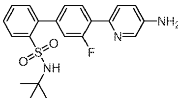
4'-(5-Aminopyridin-2-yl)-N-tert-butyl-3'-fluorobiphenyl-2-sulfonamide
