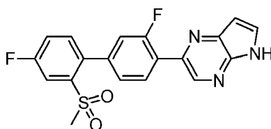
2-[3,4'-Difluoro-2'-(methylsulfonyl)biphenyl-4-yl]-5H-pyrrolo[2,3-b]pyrazine
