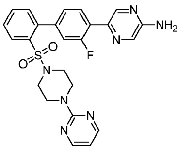
5-{3-Fluoro-2'-[(4-pyrimidin-2-yl)piperazin-1-yl)sulfonyl]biphenyl-4-yl}pyrazin-2-amine
