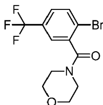
(2-Bromo-5-(trifluoromethyl)phenyl)(morpholino)methanone
