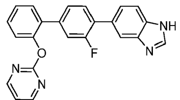
5- \{3 -Fluoro-2'-[(pyrimidin-2-yloxy)biphenyl-4-yl]-1H-benzimidazole
