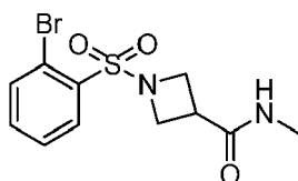
1-((2-Bromophenyl)sulfonyl)-N-methylazetidine-3-carboxamide
