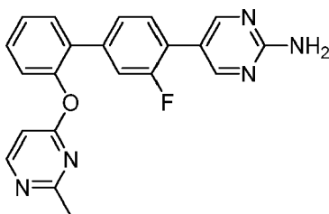
5- \{3 -Fluoro-2'-[(2-methylpyrimidin-4-yl)oxy]biphenyl-4-yl}pyrimidin-2-amine
