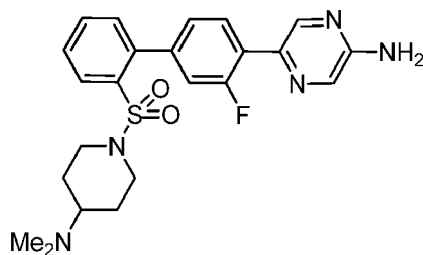
5-(2'-[4-(Dimethylamino)piperidin-1-yl]sulfonyl)-3-fluorobiphenyl-4-ylpyrazin-2-amine
