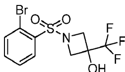
1-((2-Bromophenyl)sulfonyl)-3-(trifluoromethyl)azetidin-3-ol
