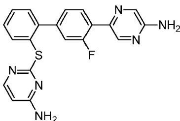
2-[[4'-(5-Aminopyrazin-2-yl)-3'-fluorobiphenyl-2-yl]sulfanyl]pyrimidin-4-amine hydrochloride
