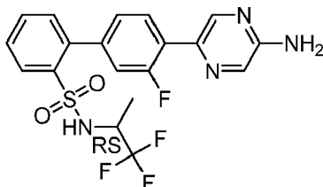
racemic 4'-(5-Aminopyrazin-2-yl)-3'-fluoro-N-(2,2,2-trifluoro-1-methylethyl)biphenyl-2-sulfonamide
