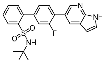
N-tert-Butyl-3'-fluoro-4'-(1H-pyrrolo[2,3-b]pyridin-5-yl)biphenyl-2-sulfonamide
