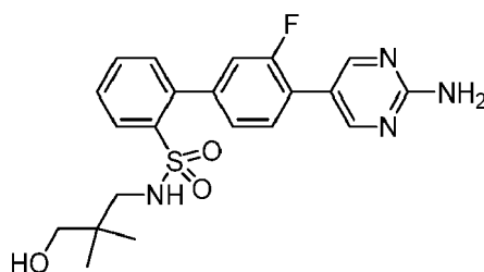
4'-(2-Aminopyrimidin-5-yl)-3'-fluoro-N-(3-hydroxy-2,2-dimethylpropyl)biphenyl-2-sulfonamide
