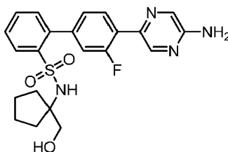
4'-(5-Aminopyrazin-2-yl)-3'-fluoro-N-[1-(hydroxymethyl)cyclopentyl]biphenyl-2-sulfonamide
