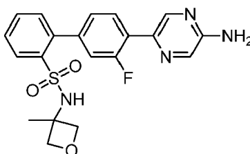
4'-(5-Aminopyrazin-2-yl)-3'-fluoro-N-(3-methyloxetan-3-yl)biphenyl-2-sulfonamide
