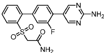
2-[[4'-(2-Aminopyrimidin-5-yl)-3'-fluorobiphenyl-2-yl]sulfonyl]acetamide.
