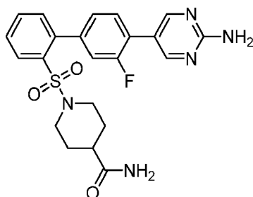
1-((4'-(2-Aminopyrimidin-5-yl)-3'-fluoro-[1,1'-biphenyl]-2-yl)sulfonyl)piperidine-4-carboxamide
