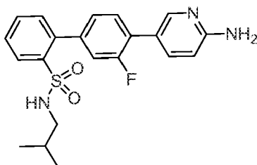
4'-(6-Aminopyridin-3-yl)-3'-fluoro-N-iso-butyl-[1,1'-biphenyl]-2-sulfonamide
