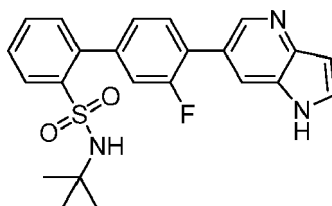
N-tert-Butyl-3'-fluoro-4'-(1H-pyrrolo[3,2-b]pyridin-6-yl)biphenyl-2-sulfonamide
