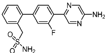
1-[4'-(5-Aminopyrazin-2-yl)-3'-fluorobiphenyl-2-yl]methanesulfonamide hydrochloride
