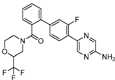
racemic 5-(3-Fluoro-2'-([2-(trifluoromethyl)morpholin-4-yl]carbonyl)biphenyl-4-yl)pyrazin-2-amine
