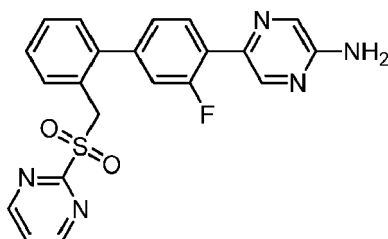
5-[3-Fluoro-2'-[(pyrimidin-2-ylsulfonyl)methyl]biphenyl-4-yl]pyrazin-2-amine
