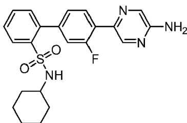
4'-(5-Aminopyrazin-2-yl)-N-cyclohexyl-3'-fluorobiphenyl-2-sulfonamide
