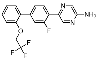
5-[3-Fluoro-2'-(2,2,2-trifluoroethoxy)biphenyl-4-yl]pyrazin-2-amine
