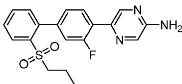
5-[3-Fluoro-2'-(propylsulfonyl)biphenyl-4-yl]pyrazin-2-amine
