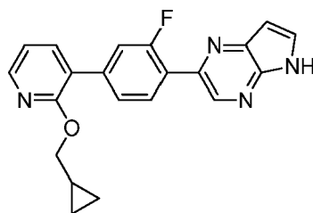
2-{4-[2-(Cyclopropylmethoxy)pyridin-3-yl]-2-fluorophenyl}-5H-pyrrolo[2,3-b]pyrazine
