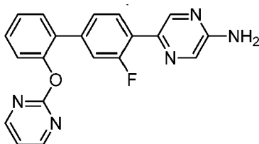
5-[3-Fluoro-2'-(pyrimidin-2-yloxy)biphenyl-4-yl]pyrazin-2-amine
