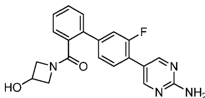
2-[4-(2-Aminopyrimidin-5-yl)-3-fluoro-phenyl]phenyl]-(3-hydroxyazetidin-1-yl)methanone
