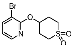
4-((3-Bromopyridin-2-yl)oxy)tetrahydro-2H-thiopyran 1,1-dioxide
