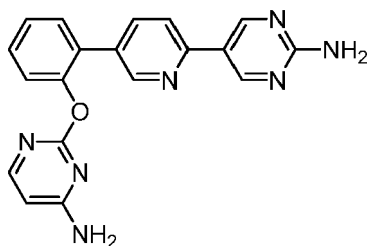
5-(5-{2-[(4-Aminopyrimidin-2-yl)oxy]phenyl}pyridin-2-yl)pyrimidin-2-amine
