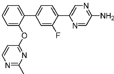
5- \{3 -Fluoro-2'-[(2-methylpyrimidin-4-yl)oxy]biphenyl-4-yl}pyrazin-2-amine
