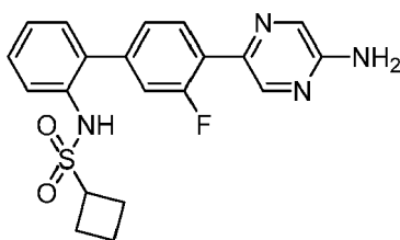
N -(4'-(5-Aminopyrazin-2-yl)-3'-fluoro-[1,1'-biphenyl]-2-yl)cyclobutanesulfonamide
