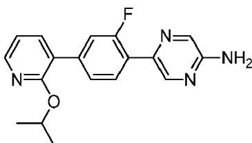
5-{2-Fluoro-4-[2-(1-methylethoxy)pyridin-3-yl]phenyl}pyrazin-2-amine
