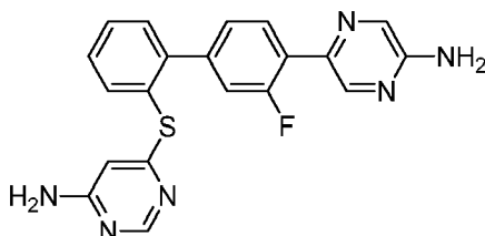
6-[[4'-(5-Aminopyrazin-2-yl)-3'-fluorobiphenyl-2-yl]sulfanyl]pyrimidin-4-amine hydrochloride
