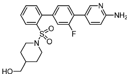
(1-((4'-(6-Aminopyridin-3-yl))-3'-fluoro-[1,1'-biphenyl]-2-yl)sulfonylpiperidin-4-yl)methanol
