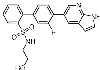
3'-Fluoro-N-(2-hydroxyethyl)-4'-(1H-pyrrolo[2,3-b]pyridin-5-yl)biphenyl-2-sulfonamide
