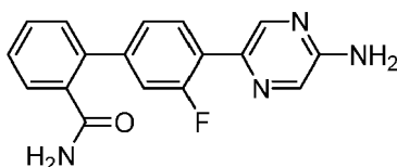
4'-(5-Aminopyrazin-2-yl)-3'-fluorobiphenyl-2-carboxamide
