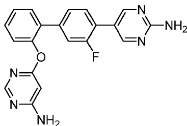
5-{2'-[(6-Aminopyrimidin-4-yl)oxy]-3-fluorobiphenyl-4-yl}pyrimidin-2-amine
