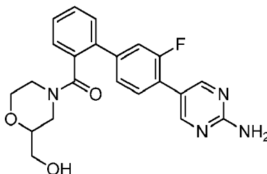
racemic [2-[4-(2-Aminopyrimidin-5-yl)-3-fluoro-phenyl]phenyl]-[2-(hydroxymethyl)morpholin-4-yl]methanone
