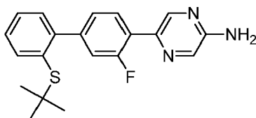
5-[2'-( tert -Butylsulfanyl)-3-fluorobiphenyl-4-yl]pyrazin-2-amine
