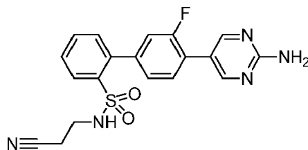
4'-(2-Aminopyrimidin-5-yl)-N-(2-cyanoethyl)-3'-fluorobiphenyl-2-sulfonamide
