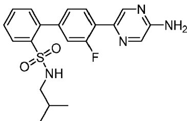
4'-(5-Aminopyrazin-2-yl)-3'-fluoro-N-(2-methylpropyl)biphenyl-2-sulfonamide
