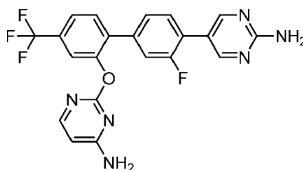
5-{2'-[(4-Aminopyrimidin-2-yl)oxy]-3-fluoro-4'-(trifluoromethyl)biphenyl-4-yl}pyrimidin-2-amine
