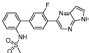
N -[3'-Fluoro-4'-(5H-pyrrolo[2,3-b]pyrazin-2-yl)biphenyl-2-yl]methanesulfonamide
