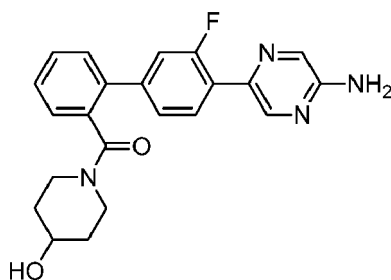
1-[[4'-(5-Aminopyrazin-2-yl)-3'-fluorobiphenyl-2-yl]carbonyl]piperidin-4-ol
