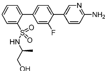
(S)-4'-(6-Aminopyridin-3-yl)-3'-fluoro-N-(1-hydroxypropan-2-yl)-[1,1'-biphenyl]-2-sulfonamide
