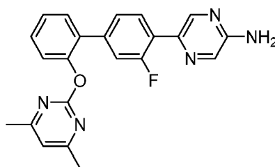
5-{2'-[(4,6-Dimethylpyrimidin-2-yl)oxy]-3-fluorobiphenyl-4-yl}pyrazin-2-amine.
