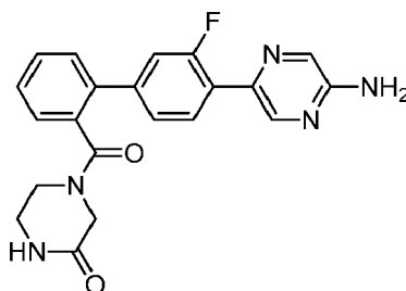
4-[[4'-(5-Aminopyrazin-2-yl)-3'-fluorobiphenyl-2-yl]carbonyl]piperazin-2-one
