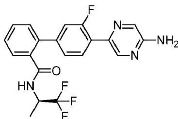
4'-(5-Aminopyrazin-2-yl)-3'-fluoro-N-[(1R)-2,2,2-trifluoro-1-methylethyl]biphenyl-2-carboxamide
