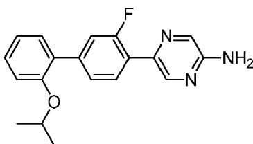
5-[3-Fluoro-2'-(1-methylethoxy)biphenyl-4-yl]pyrazin-2-amine
