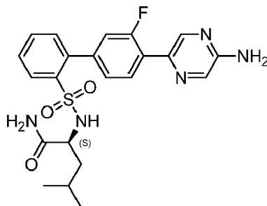
(S)-2-(4'-(5-Aminopyrazin-2-yl)-3'-fluoro-[1, 1'-biphenyl]-2-ylsulfonamido)-4-methylpentanamide
