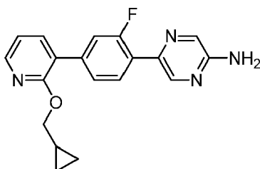
5-{4-[2-(Cyclopropylmethoxy)pyridin-3-yl]-2-fluorophenyl}pyrazin-2-amine
