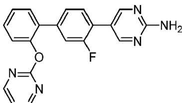
5-[3-Fluoro-2'-(pyrimidin-2-yloxy)biphenyl-4-yl]pyrimidin-2-amine
