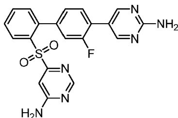
5-{2'-[(6-Aminopyrimidin-4-yl)sulfonyl]-3-fluorobiphenyl-4-yl}pyrimidin-2-amine
