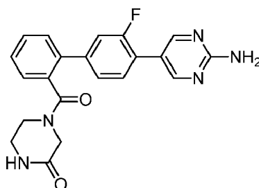
4-[[4'-(2-Aminopyrimidin-5-yl)-3'-fluorobiphenyl-2-yl]carbonyl]piperazin-2-one
