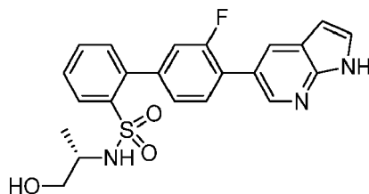
3'-Fluoro-N-[(1S)-2-hydroxy-1-methylethyl]-4'-(1H-pyrrolo[2,3-b]pyridin-5-yl)biphenyl-2-sulfonamide
