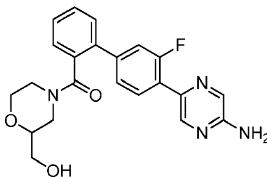
racemic [2-[4-(5-Aminopyrazin-2-yl)-3-fluoro-phenyl]phenyl]-[2-(hydroxymethyl)morpholin-4-yl]methanone
