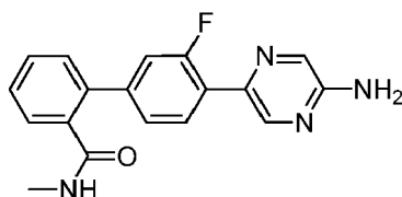
4'-(5-Aminopyrazin-2-yl)-3'-fluoro-N-methylbiphenyl-2-carboxamide
