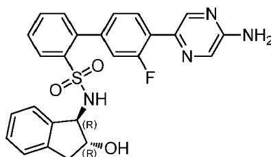
4'-(5-Aminopyrazin-2-yl)-3'-fluoro-N-((1R,2R)-2-hydroxy-2,3-dihydro-1H-inden-1-yl)-[1,1'-biphenyl]-2-sulfonamide
