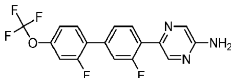
5-[2',3-Difluoro-4'-(trifluoromethoxy)biphenyl-4-yl]pyrazin-2-amine
