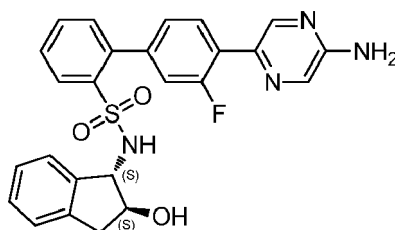
4'-(5-Aminopyrazin-2-yl)-3'-fluoro-N-((1S,2S)-2-hydroxy-2,3-dihydro-1H-inden-1-yl)-[1,1'-biphenyl]-2-sulfonamide
