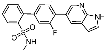
3'-Fluoro-N-methyl-4'-(1H-pyrrolo[2,3-b]pyridin-5-yl)biphenyl-2-sulfonamide
