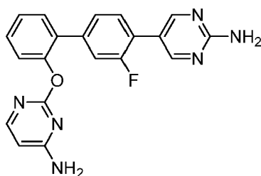
5-{2'-[(4-Aminopyrimidin-2-yl)oxy]-3-fluorobiphenyl-4-yl}pyrimidin-2-amine
