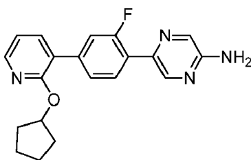
5-{4-[2-(Cyclopentylloxy)pyridin-3-yl]-2-fluorophenyl}pyrazin-2-amine
