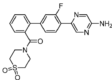
5-{2'-[(1,1-Dioxidothiomorpholin-4-yl)carbonyl]-3'-fluorobiphenyl-4-yl}pyrazin-2-amine
