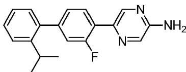
5-[3-Fluoro-2'-(1-methylethyl)biphenyl-4-yl]pyrazin-2-amine
