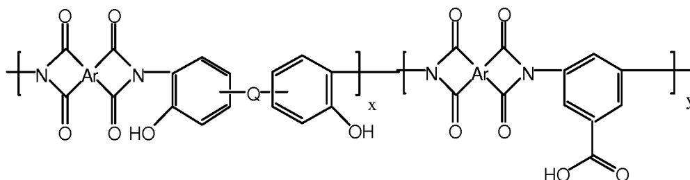
<Structural Formula 1>
