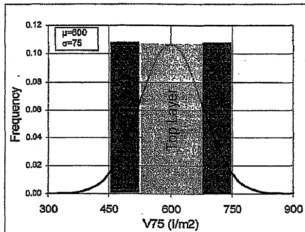
Figure 3. Strategy "A" for membrane layering.
