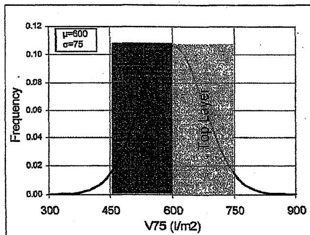
Figure 4. Strategy "B" for membrane layering.
