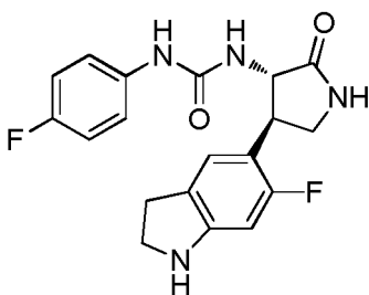
(-)-1-((3S*,4R*)-4-(6-Fluoroindolin-5-yl)-2-oxopyrrolidin-3-yl)-3-(4-fluorophenyl) urea
