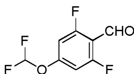
4-(Difluoromethoxy)-2,6-difluorobenzaldehyde
