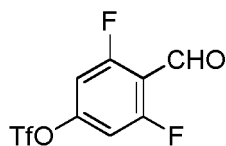
3,5-Difluoro-4-formylphenyl trifluoromethanesulfonate
