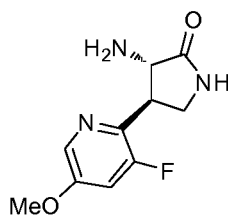
(3S*,4R*)-3-Amino-4-(3-fluoro-5-methoxypyridin-2-yl)pyrrolidin-2-one
