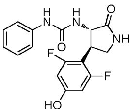
1-((3S*,4R*)-4-(2,6-Difluoro-4-hydroxyphenyl)-2-oxopyrrolidin-3-yl)-3-phenylurea
