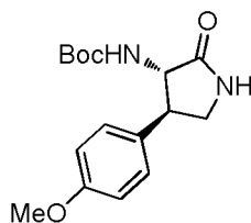
(-)-[(3S*,4R*)-4-(4-Methoxyphenyl)-2-oxopyrrolidin-3-yl]carbamic acid tert-butyl ester
