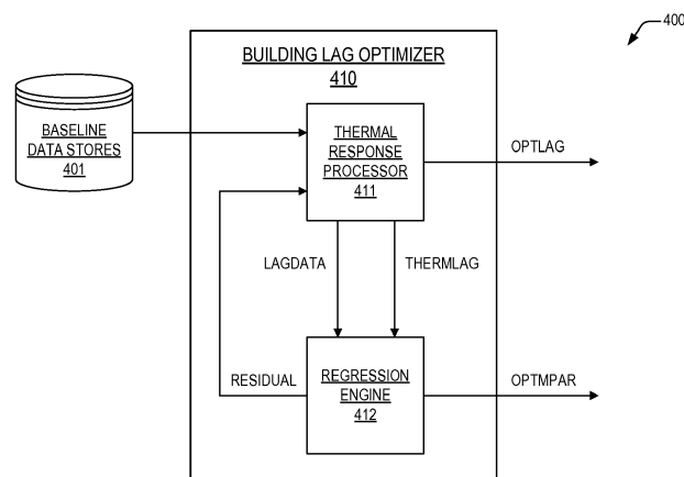
FIG. 4 FINE-GRAINED BASELINE ENERGY DATA WEATHER NORMALIZATION APPARATUS
