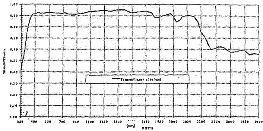
Transmittance of Sol-Gel
