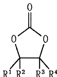
[Chemical Formula 1]
