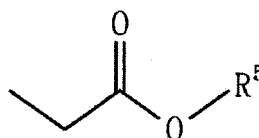
[Chemical Formula 2]
