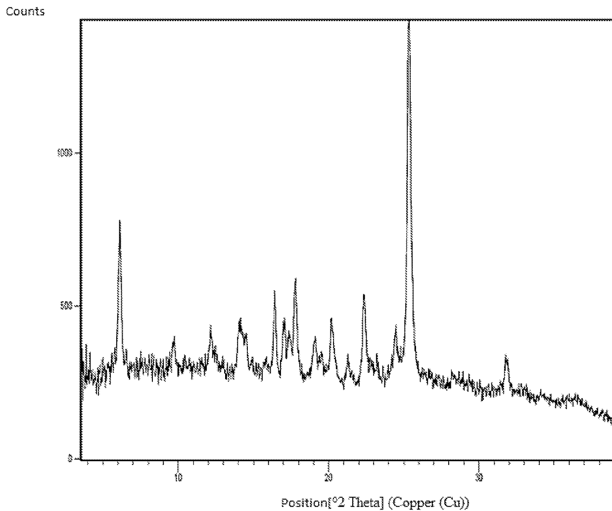
FIGURE 1c: XRPD Compound I-1 (anhydrous form A)
