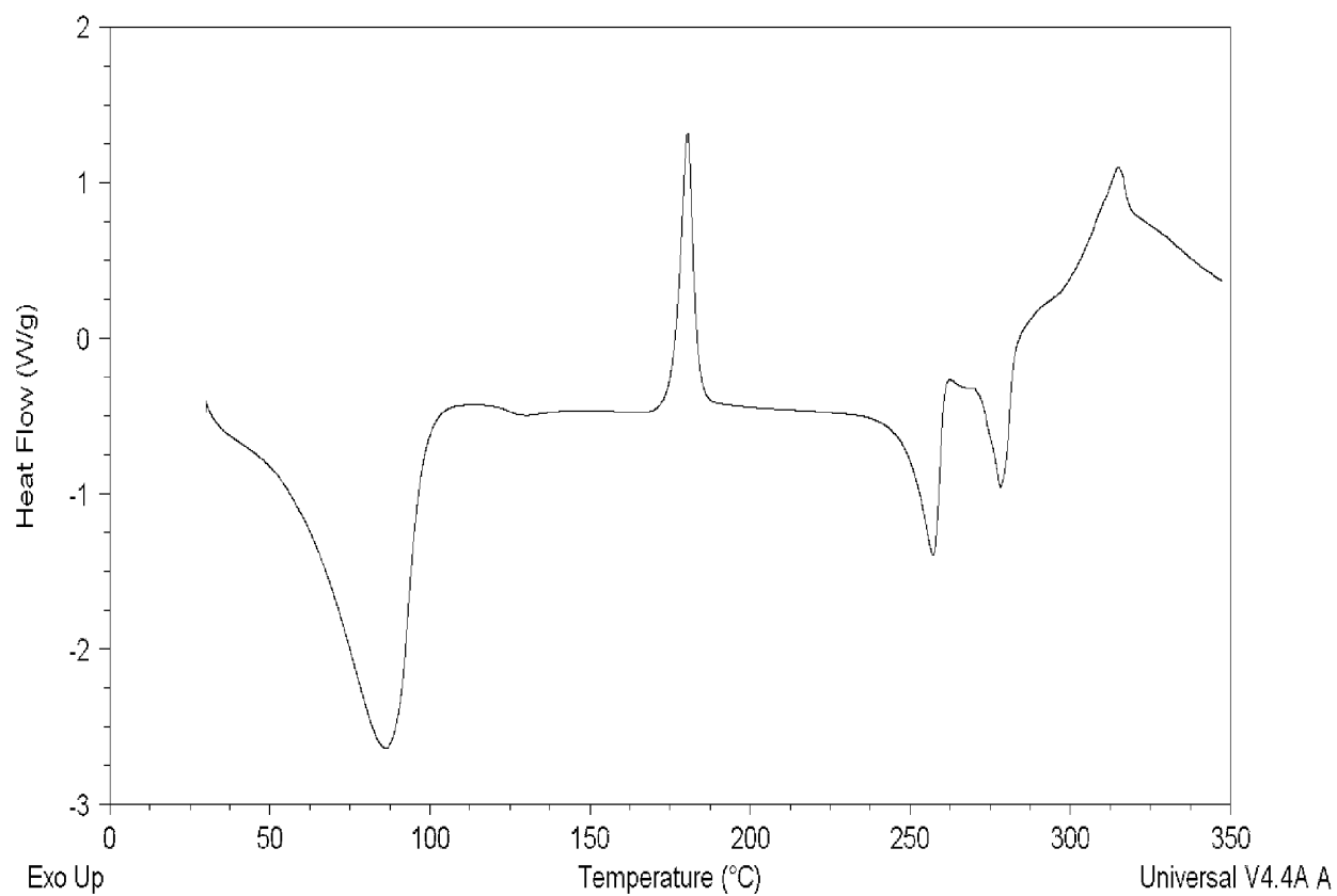
FIGURE 3b: DSC Compound I-1 (hydrate I)
