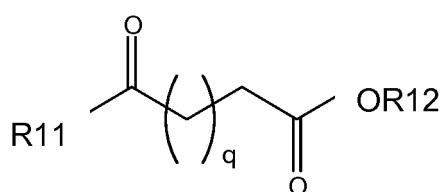
Formula VI
