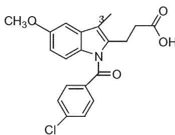
Compound 2
