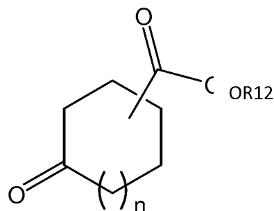
Formel VII
