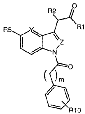
Formula I
