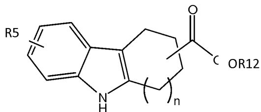
Formel IX
