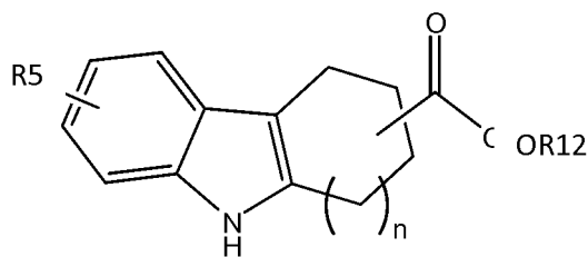
Formula IX
