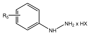
10 Formula V
