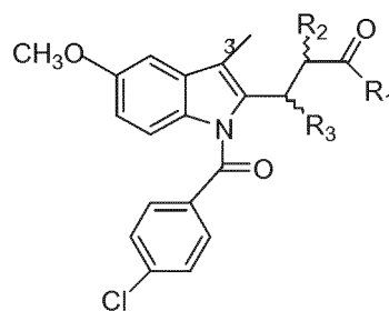
3-Methyl-indometacin analogs
