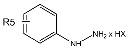
Formula V
