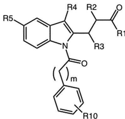
40 45 Formula II,
