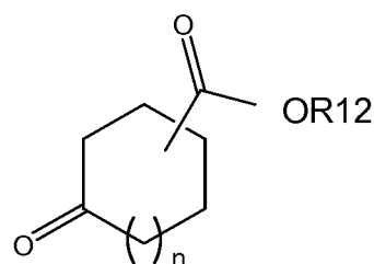
Formula VII
