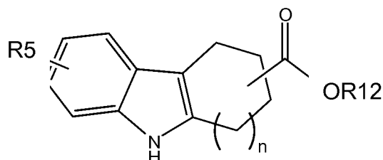
Formula IX
