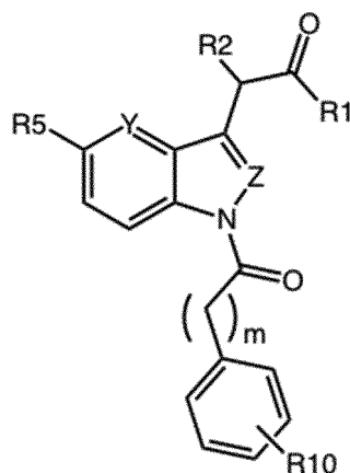
Formula I
