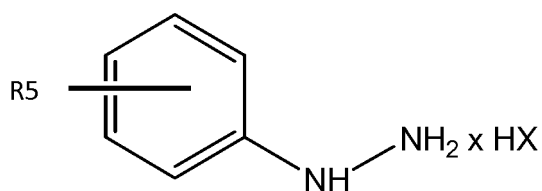
Formula V
