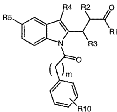
Formel II,
