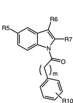
Formula III
