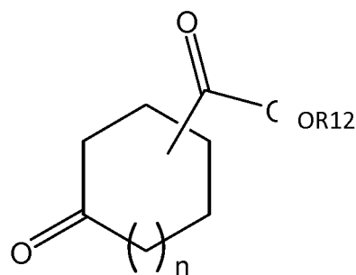
Formula VII
