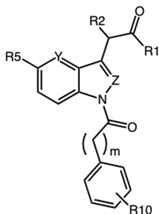
Formula I
