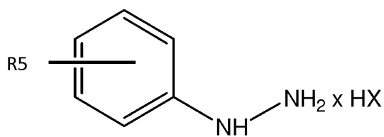
Formel V
