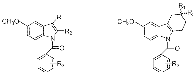
Compound 4, 5 Series
