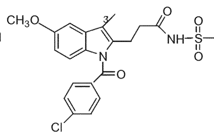
Compound 3
