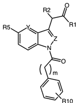
Formula I
