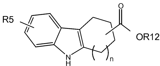
Formula IX
