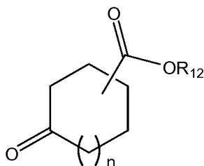
35 Formula VII
