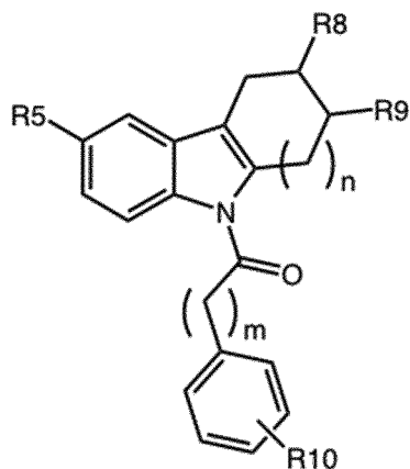
Formula III
