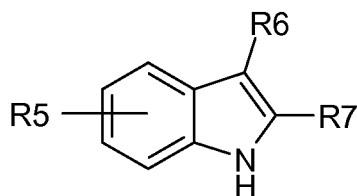
Formula VIII
