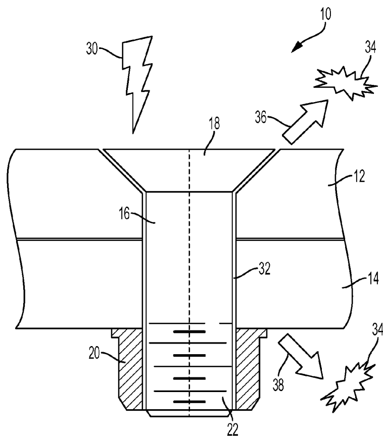
FIG. 2 PRIOR ART
