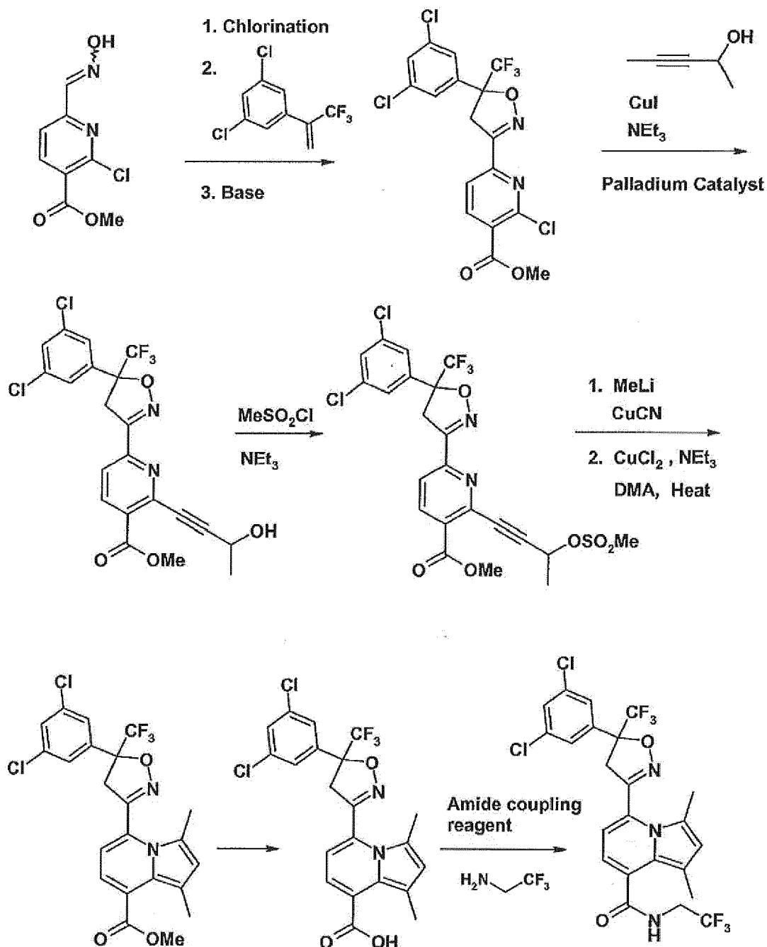
Scheme 7
