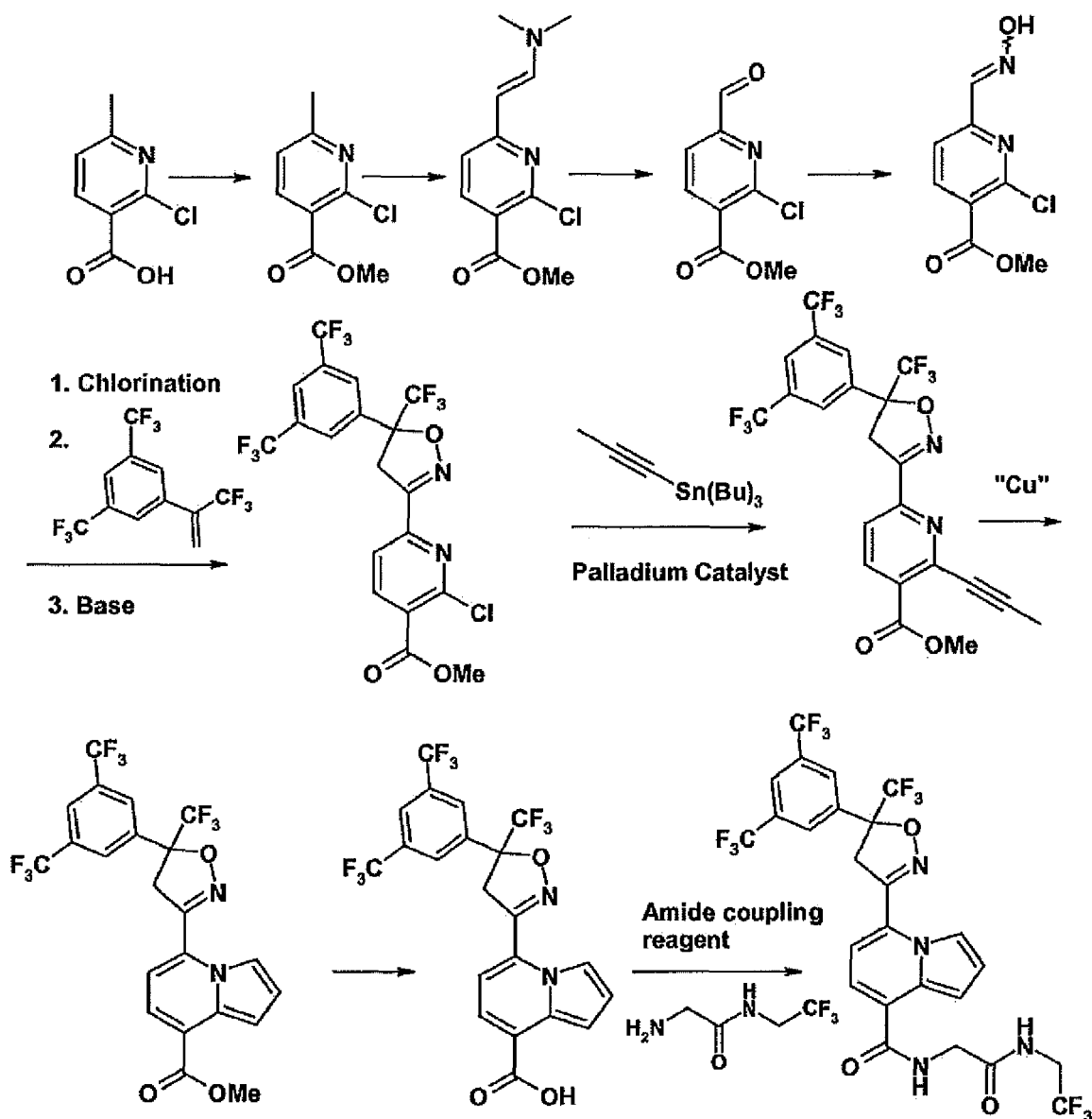
Scheme 4
