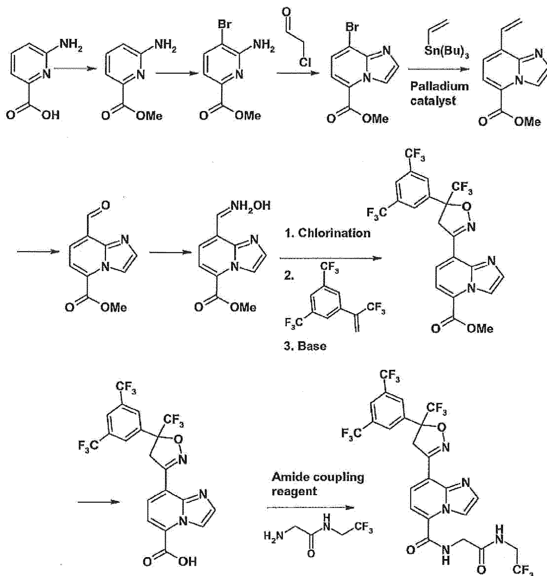
Scheme 6
