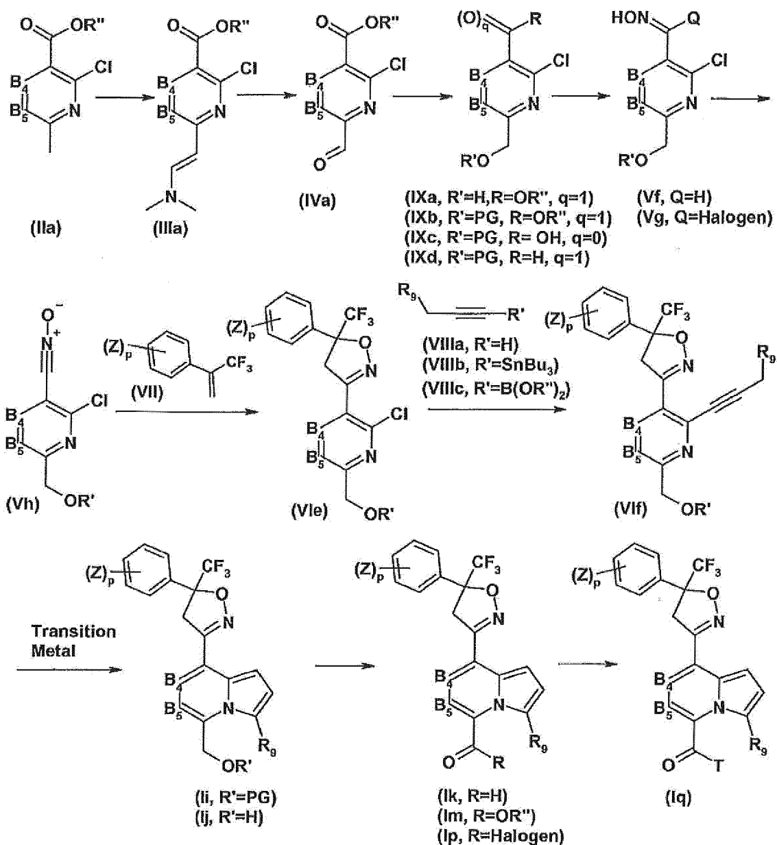
Scheme 3
