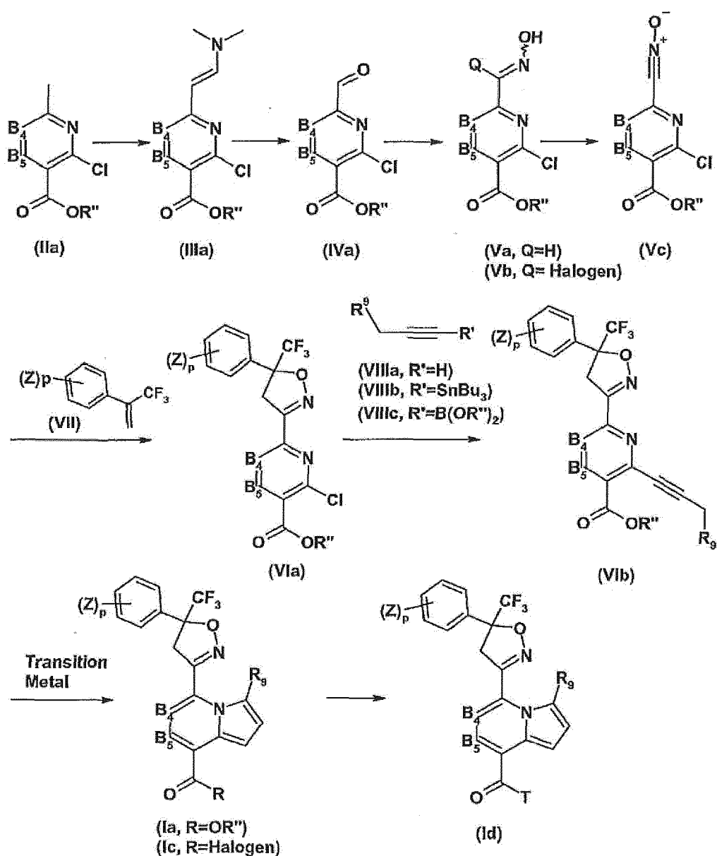
Scheme 1
