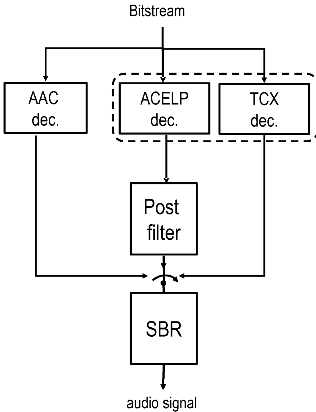
Fig. 2 (prior art)
