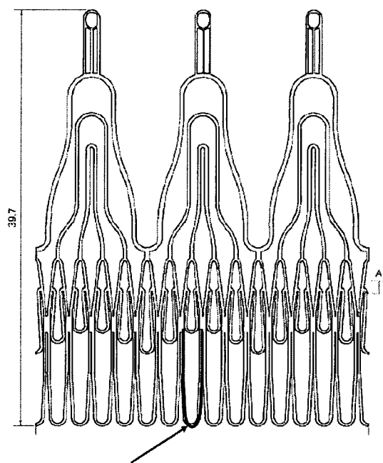
Single strut configuration 102
