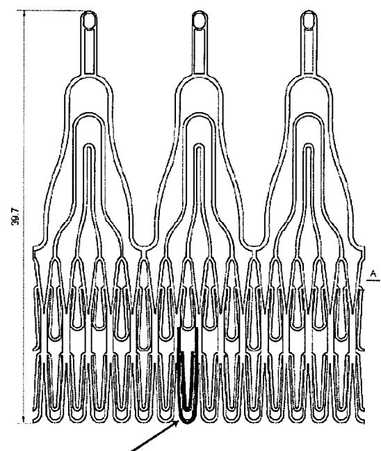
Double strut configuration 202 204
